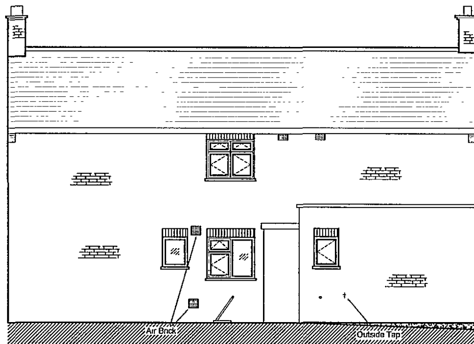
NORTH ELEVATION
