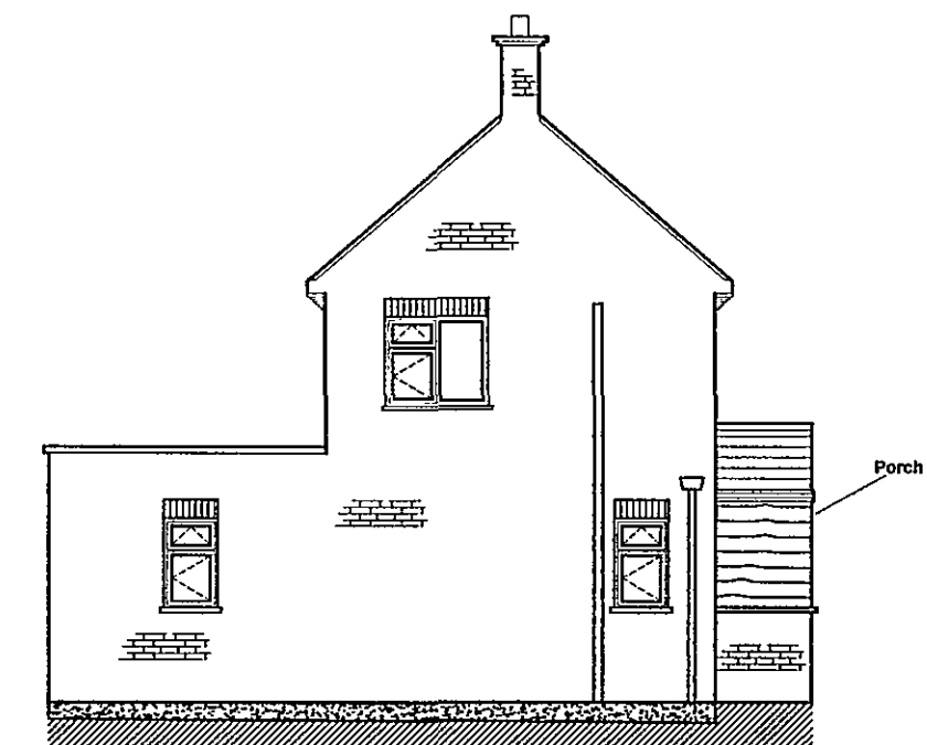
WEST ELEVATION
