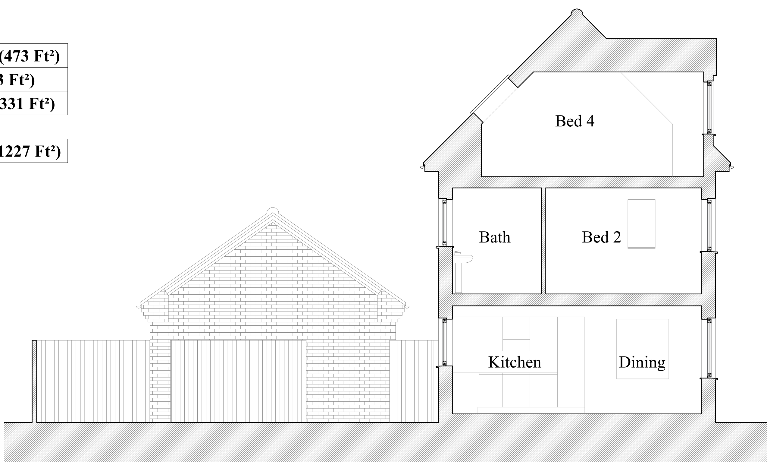
2 TYPICAL SECTION 1:50 @ A1 (1:100 @ A3)
