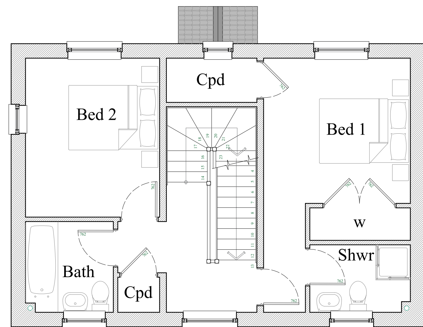
4 FIRST FLOOR PLAN 1:50 @ A1 (1:100 @ A3)
