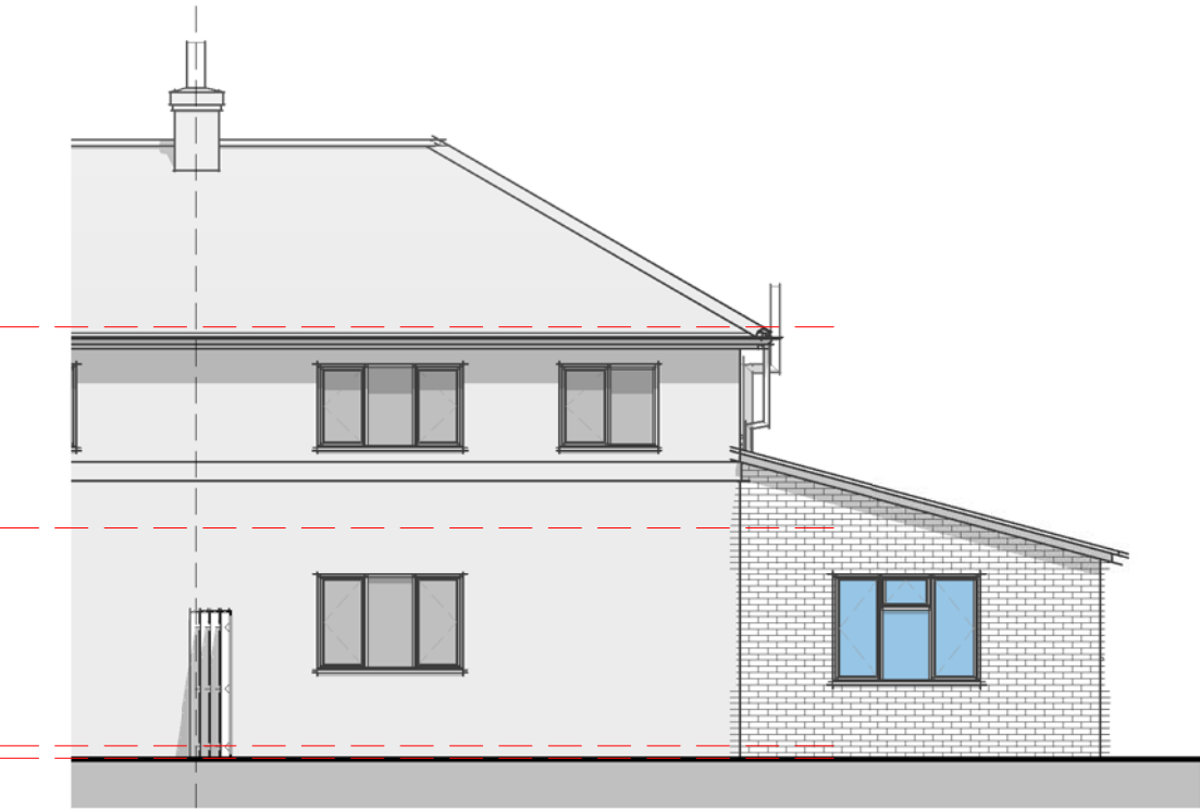
Elevation 03 - Rear 1 : 100
