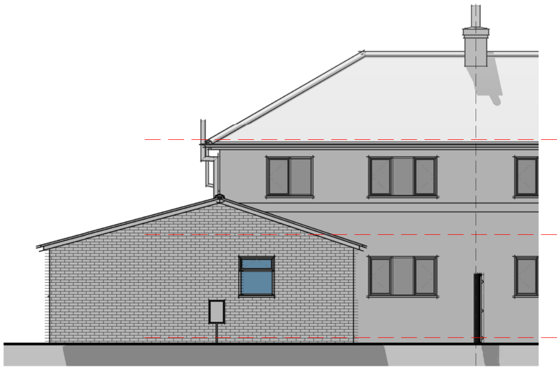
Elevation 01 - Front 1 : 100
