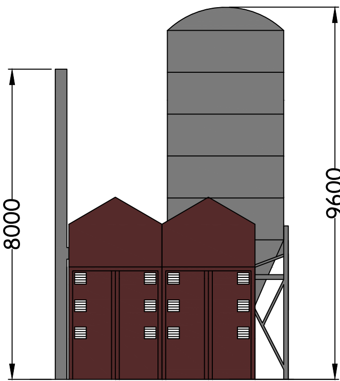
North Elevation
