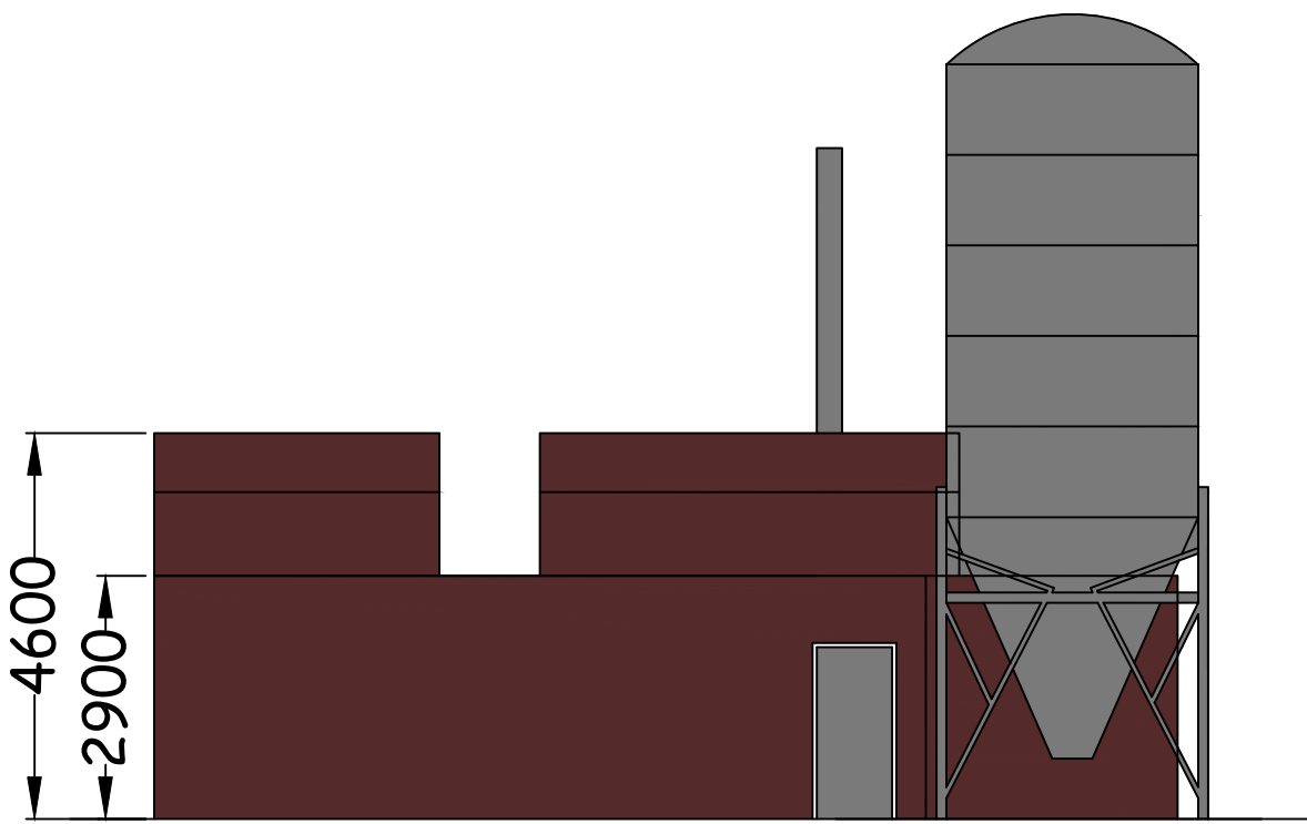
West Elevation
