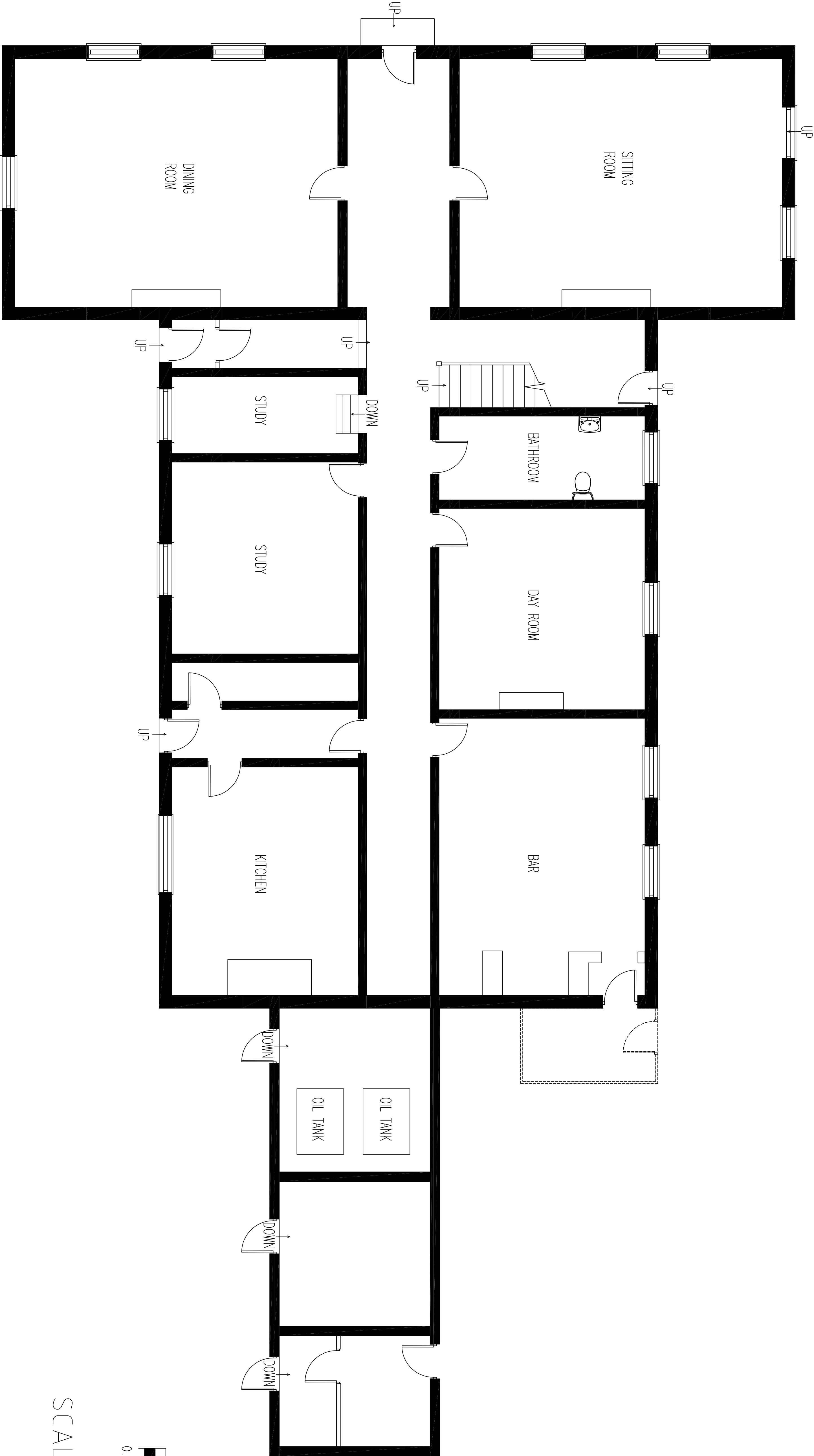
DEMOLITIONS PLAN @1:50
