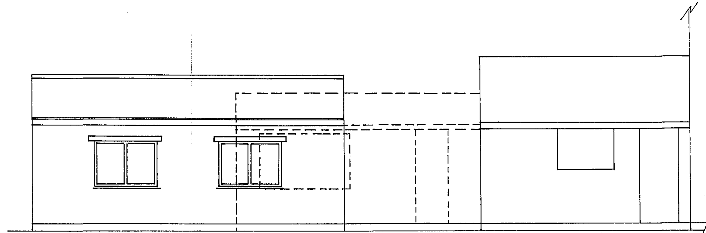
EXISTING / PROPOSED ELEVATION 1:50
