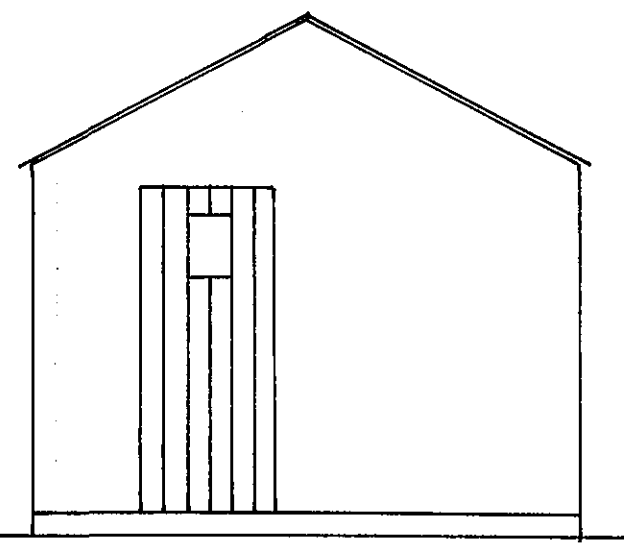
PROPOSED SIDE ELEVATION 1:50
