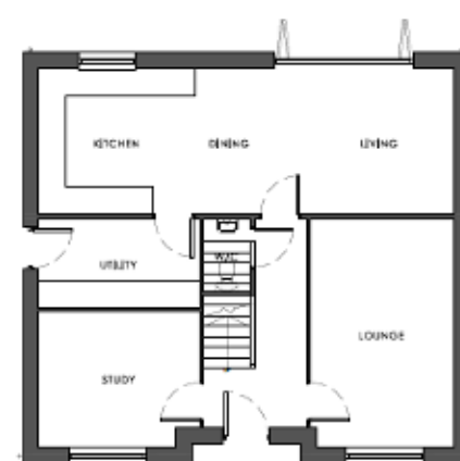
GROUND FLOOR Gross external floor area - 83m² Gross internal floor area - 74m²
