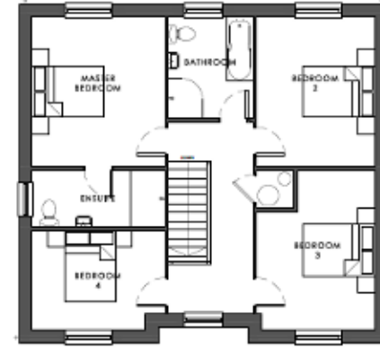
FIRST FLOOR Gross external floor area - 83m² Gross internal floor area - 74m²
