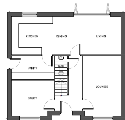
GROUND FLOOR Gross external floor area - 80m² Gross internal floor area - 74m²
