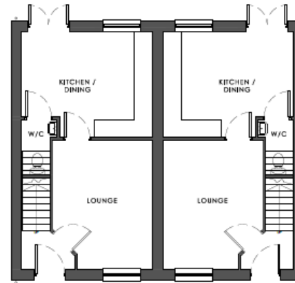
GROUND FLOOR Gross external floor area - 83m² units combined Gross internal floor area - 34m² per unit
