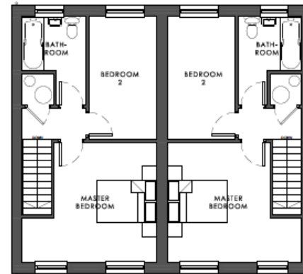
FIRST FLOOR Gross external floor area - 83m² units combined Gross internal floor area - 34m² per unit
