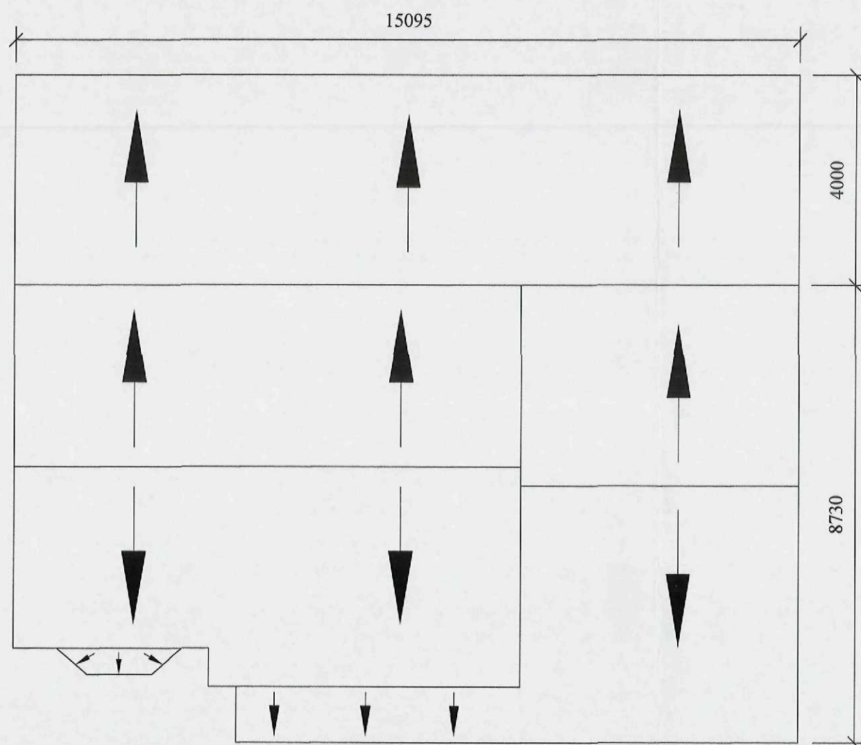
PROPOSED ROOF LAYOUT
