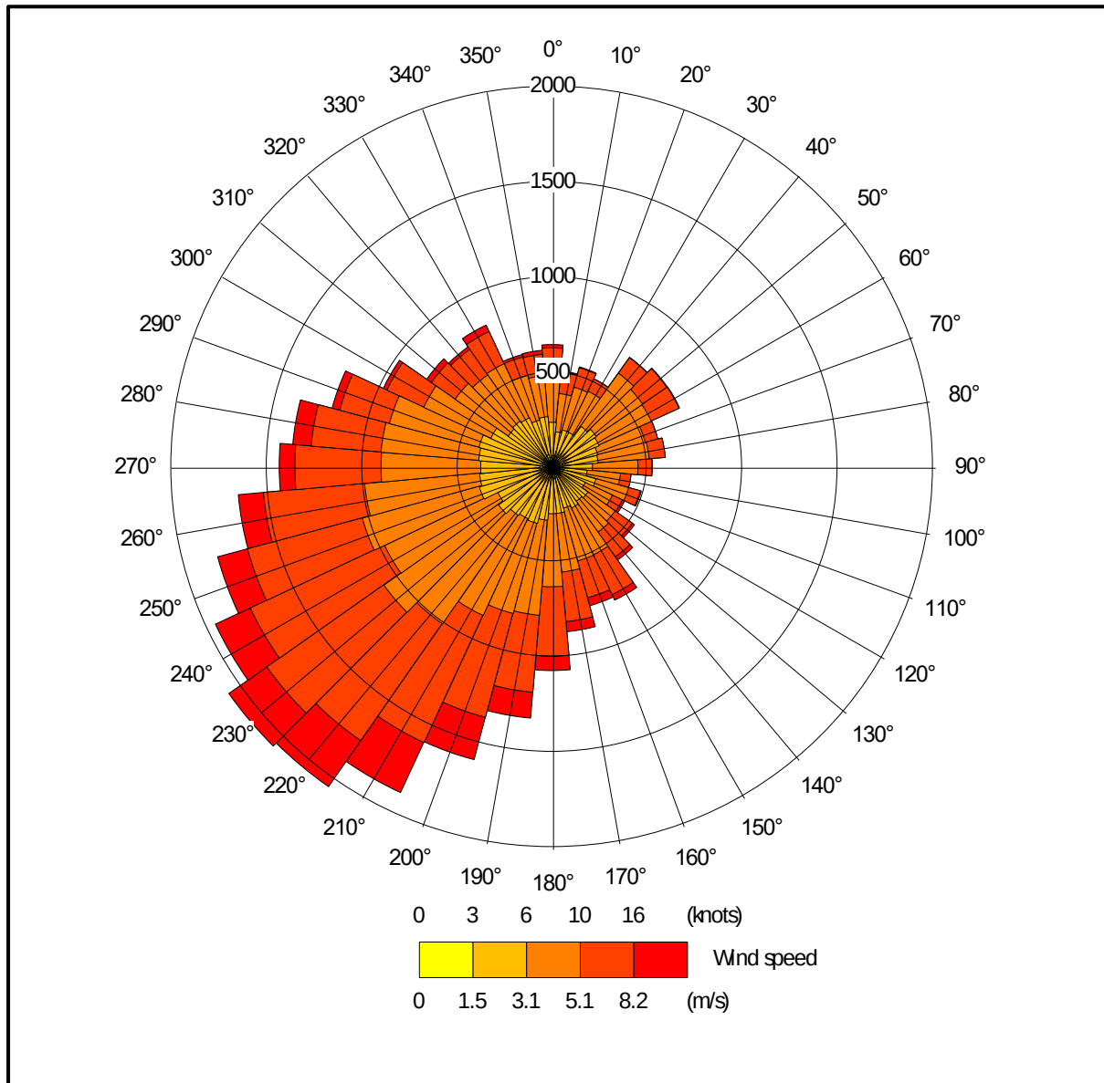
Figure 3a. The wind rose. GFS derived data, for 52.736 N, 0.293 W, 2014 - 2017
