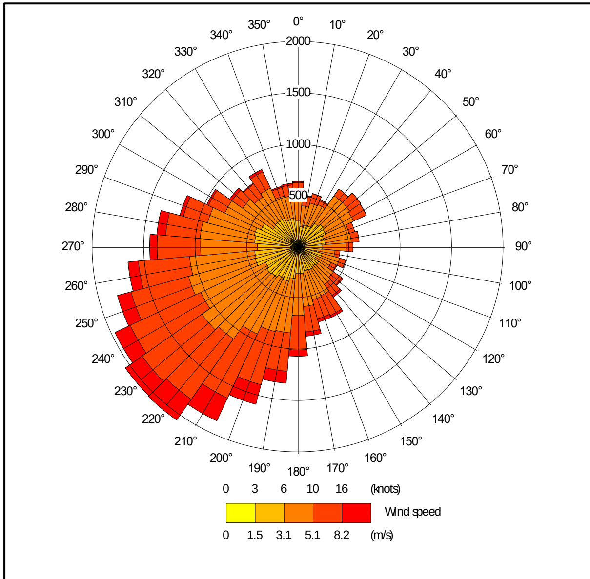
Figure 3b. The wind rose. FLOWSTAR modified GFS derived data NGR 515250, 316750, 2014-2017
