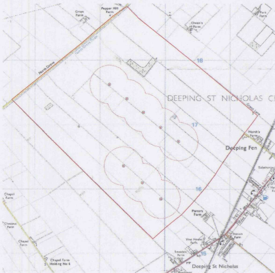
Figure 1. The proposed breeding bird monitoring programme study area. The solid red line indicate the boundary of the proposed monitoring study area, the red dashed line the area within 300m of the wind turbines (which are shown as red and black circles).
