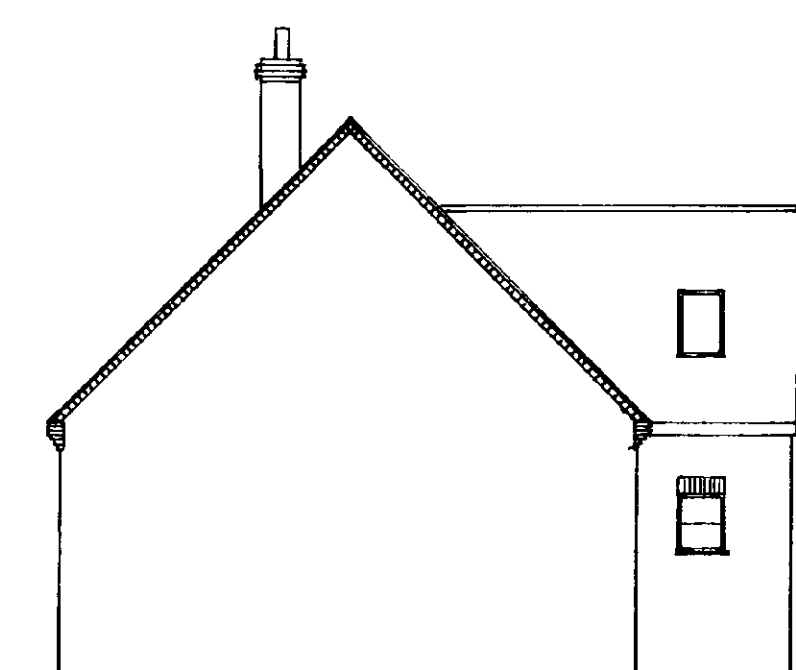
HOUSE TYPE "B" PROPOSED SIDE ELEVATION SCALE 1:100
