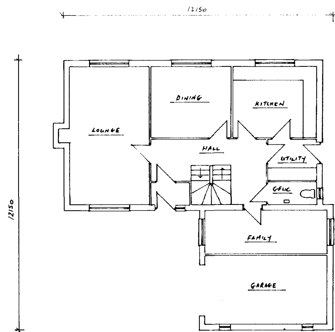
HOUSE TYPE "A" PROPOSED GROUND FLOOR SCALE 1:100
