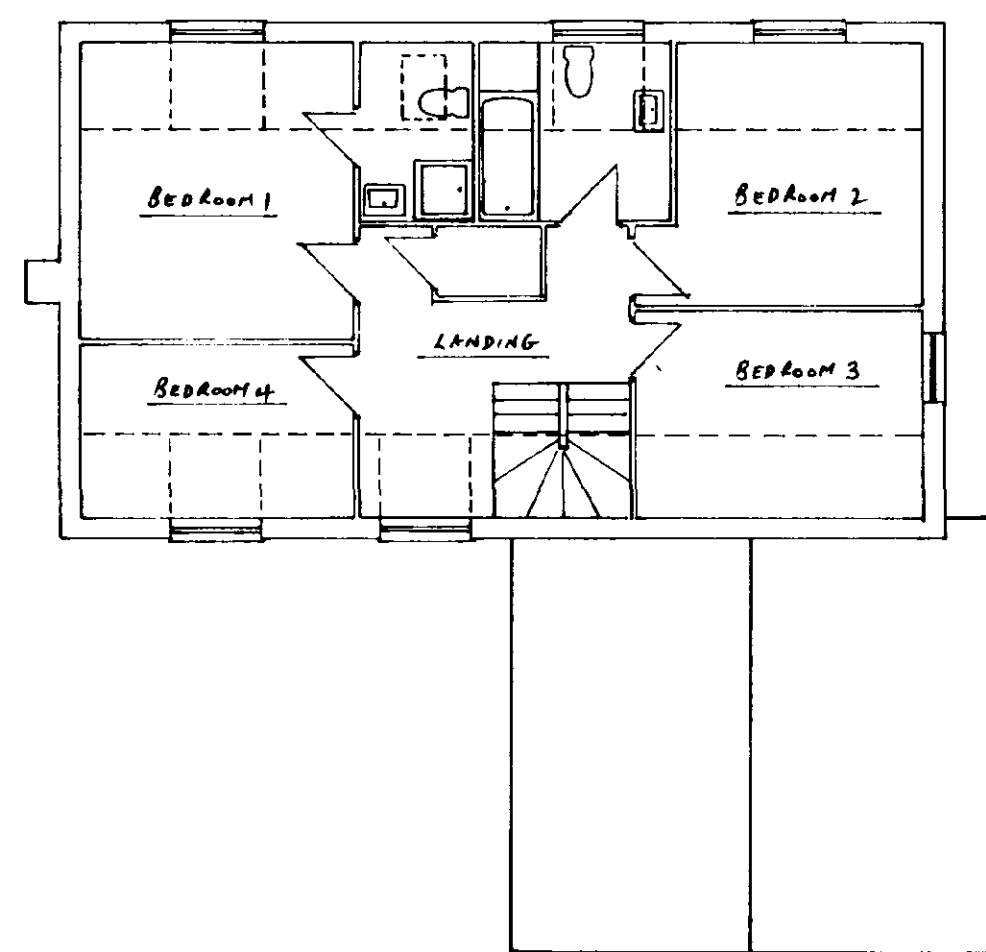
HOUSE TYPE "A" PROPOSED FIRST FLOOR SCALE 1:100
