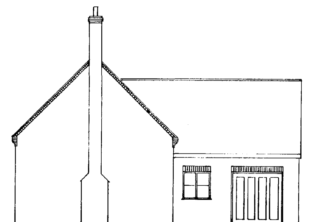
HOUSE TYPE "A" PROPOSED SIDE ELEVATION SCALE 1:100
