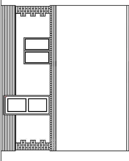
PROPOSED SIDE ELEVATION 1:100
