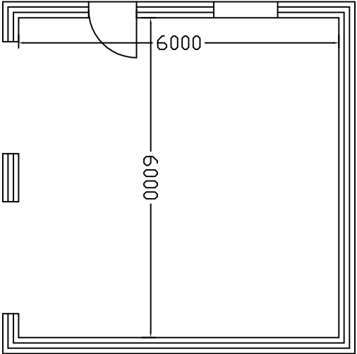
PROPOSED GROUND FLOOR LAYOUT 1:100
