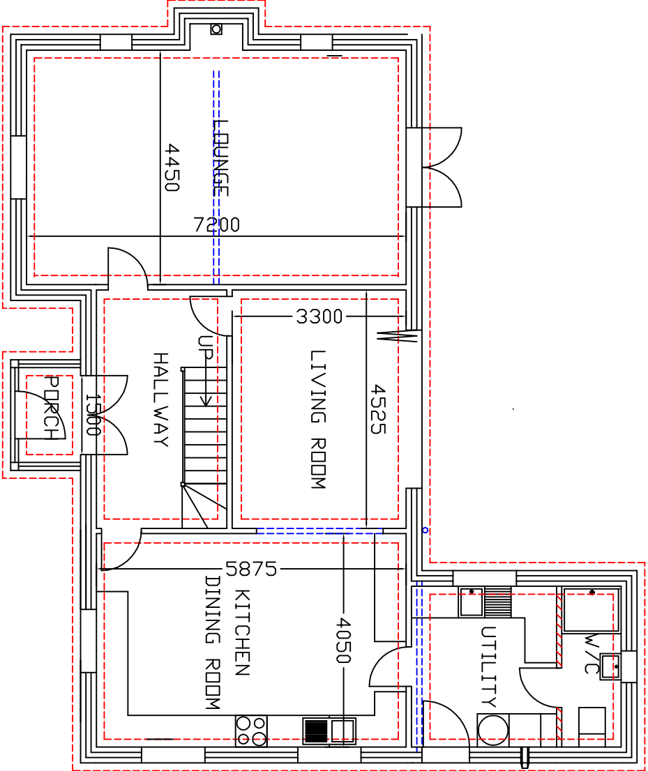
PROPOSED GROUND FLOOR LAYOUT 1:50
