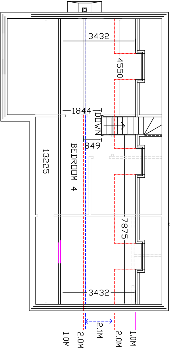
PROPOSED SECOND FLOOR LAYOUT 1:50
