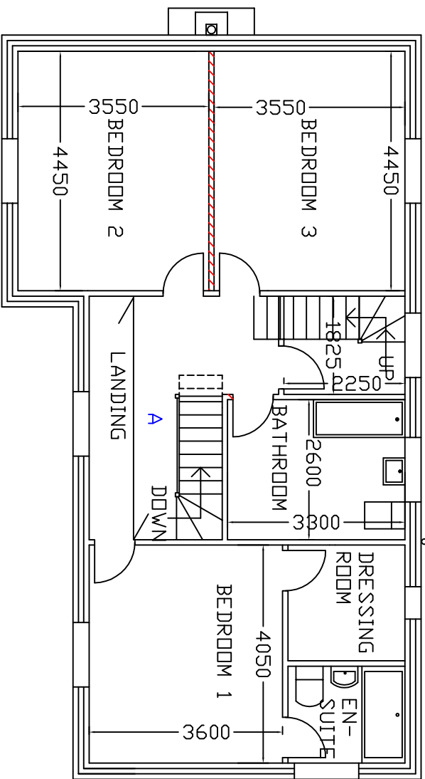
PROPOSED FIRST FLOOR LAYOUT 1:50
