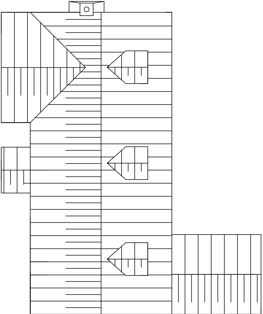
PROPOSED ROOF LAYOUT 1:50
