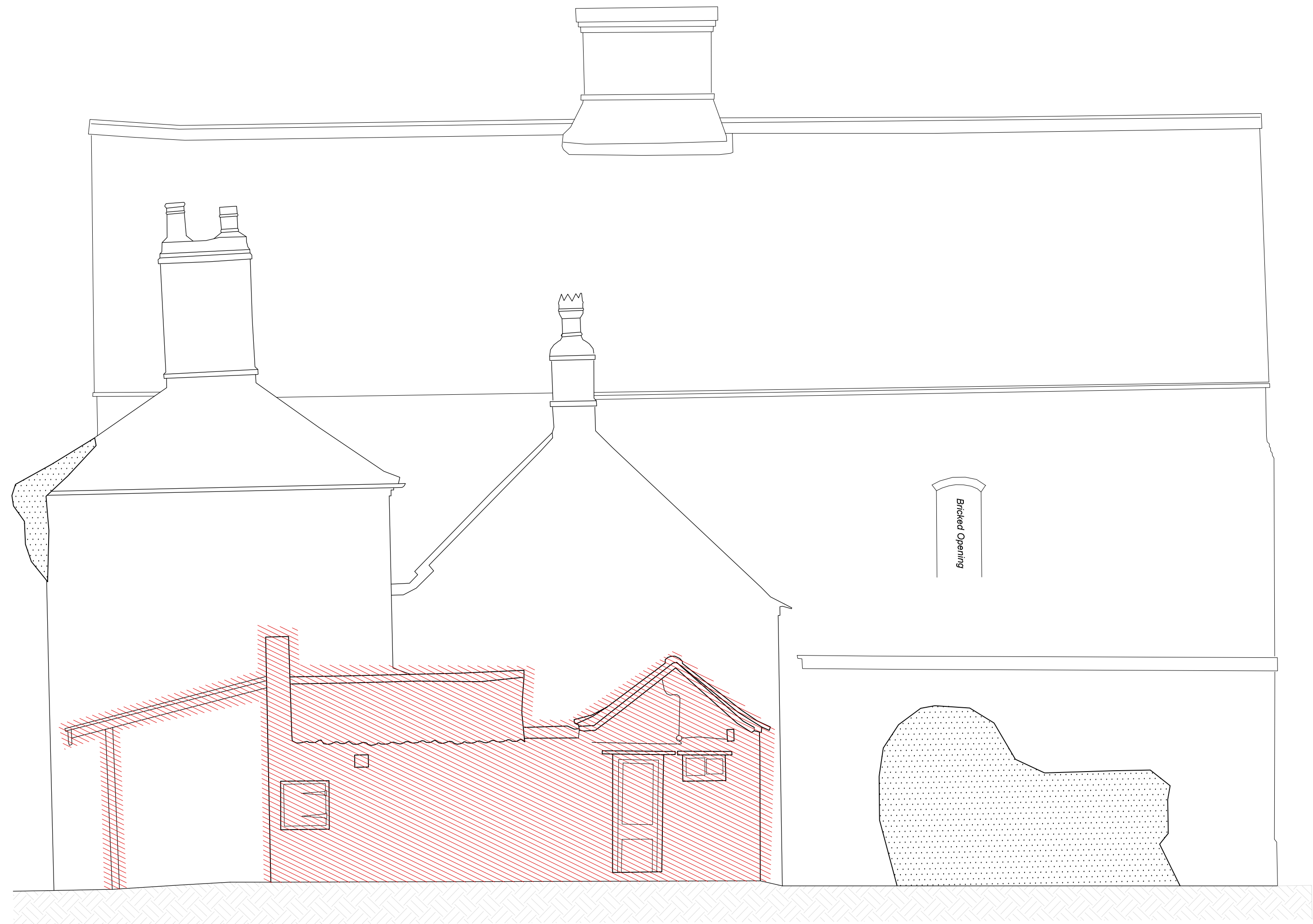
PROPOSED DEMOLITION ELEVATION B
