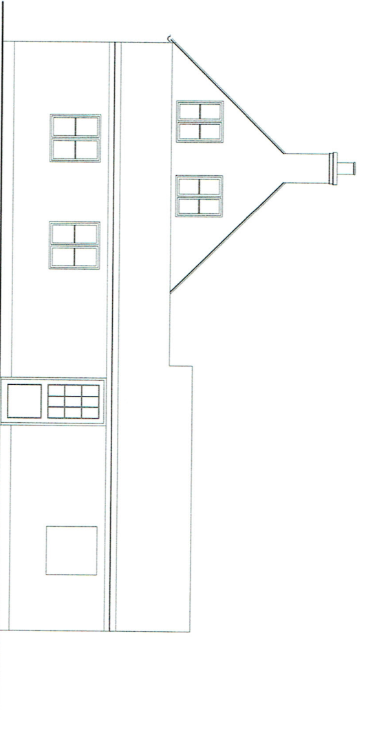
side elevation ( south ) - as existing
