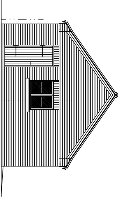
SIDE ELEVATION.
