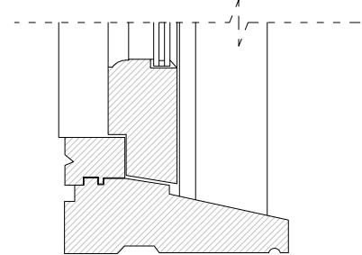
WINDOWSILL DETAIL @ 1:5
