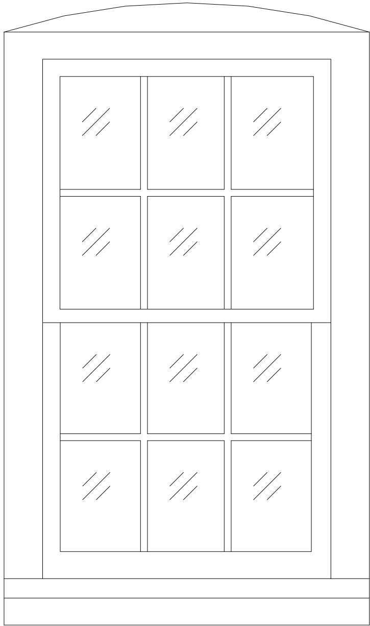
SASH WINDOW ELEVATION DETAIL @ 1:10
