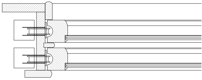
JAMB DETAIL @ 1:5
