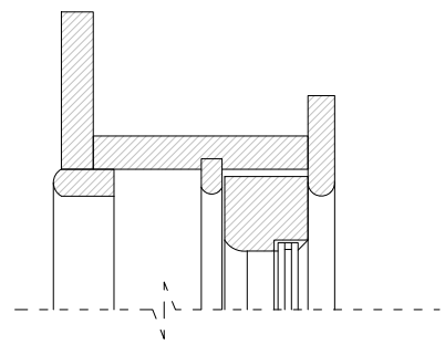
HEADER DETAIL @ 1:5
