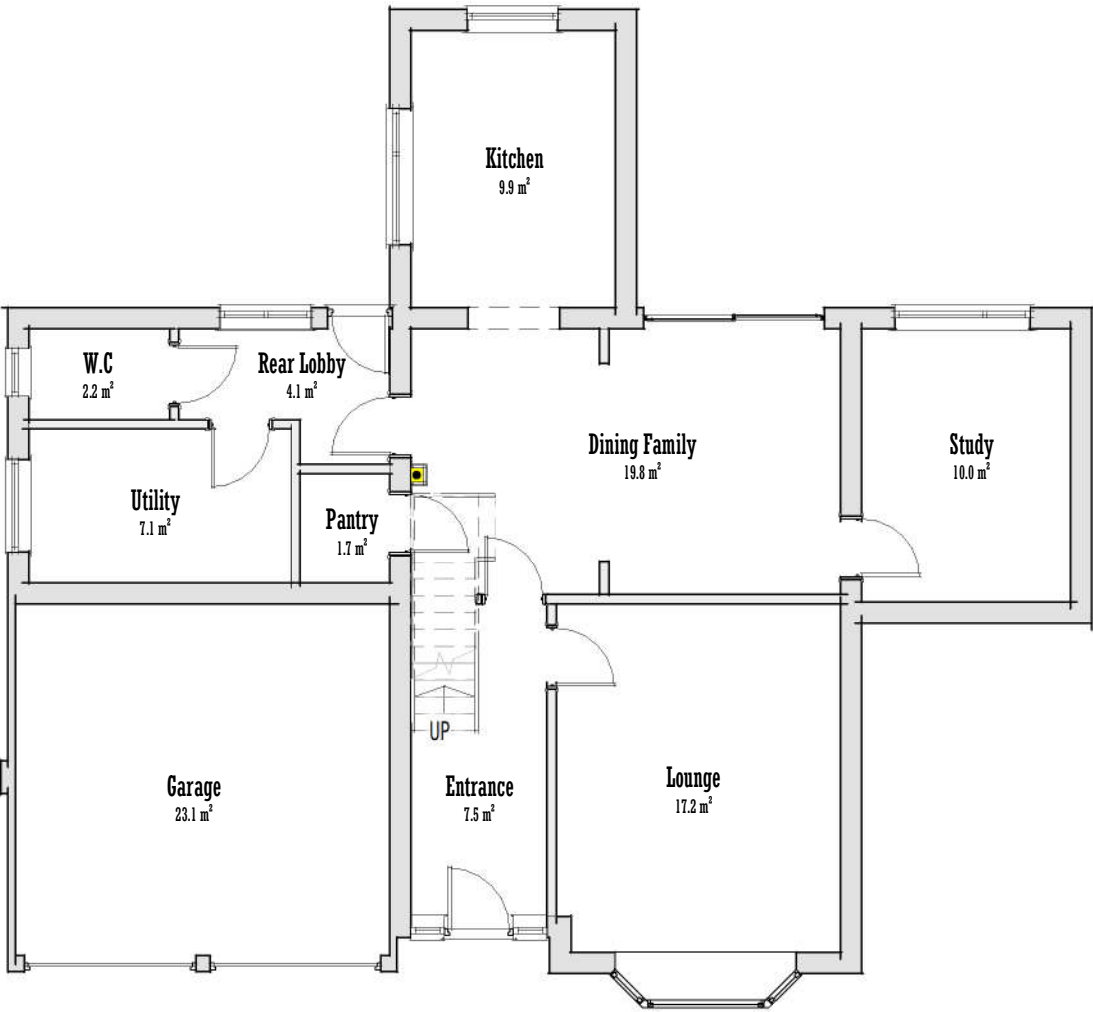
Plan 01 - Ground 1 : 100
