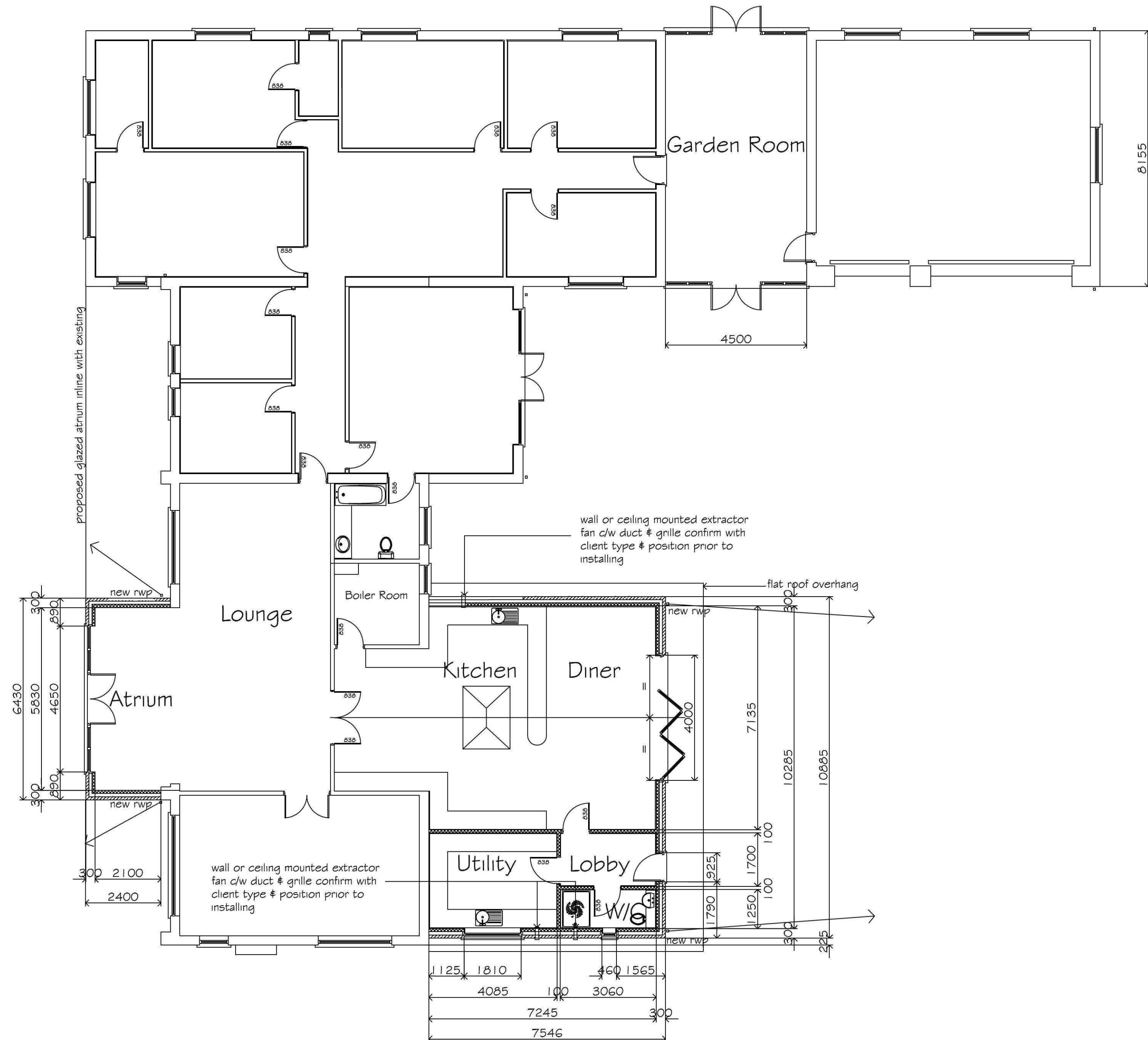
A Existing / Proposed Ground Floor Plan
