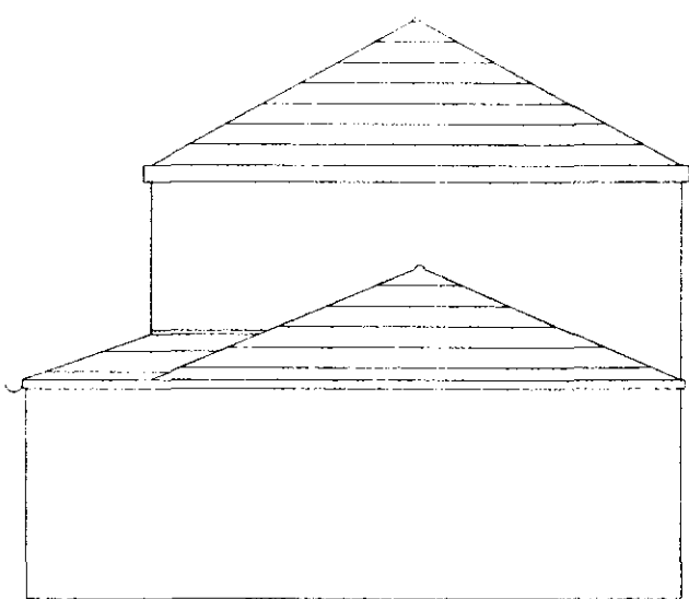
Proposed Flank Elevation
