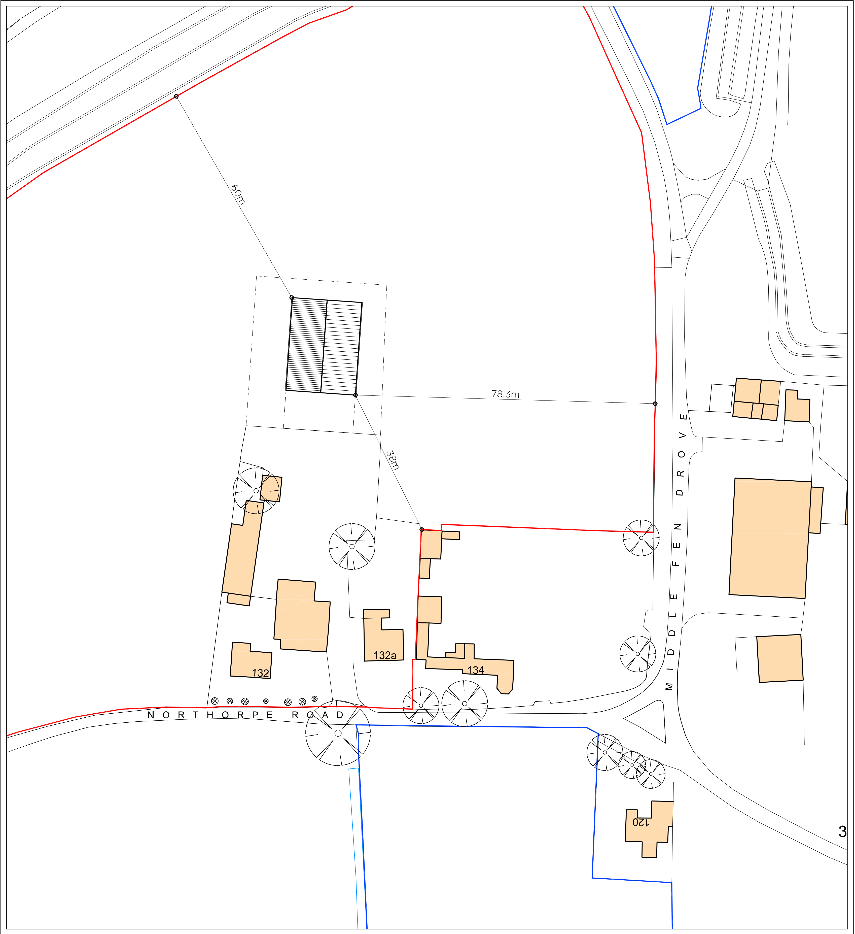
Proposed Site Layout Scale 1:500
