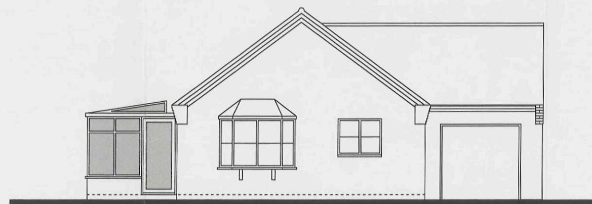
Front Elevation
