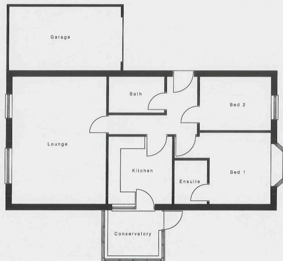
Part Ground Floor Plan
