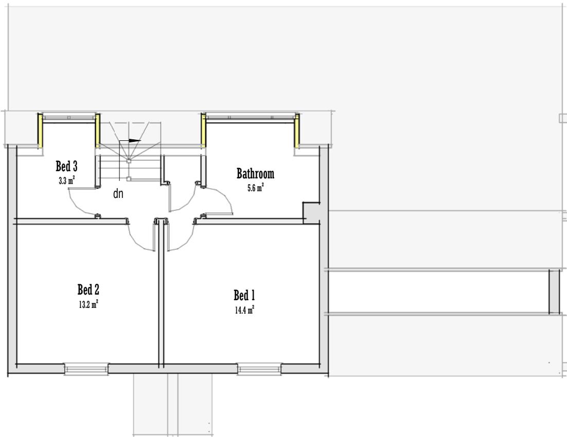
Plan 02 - First
