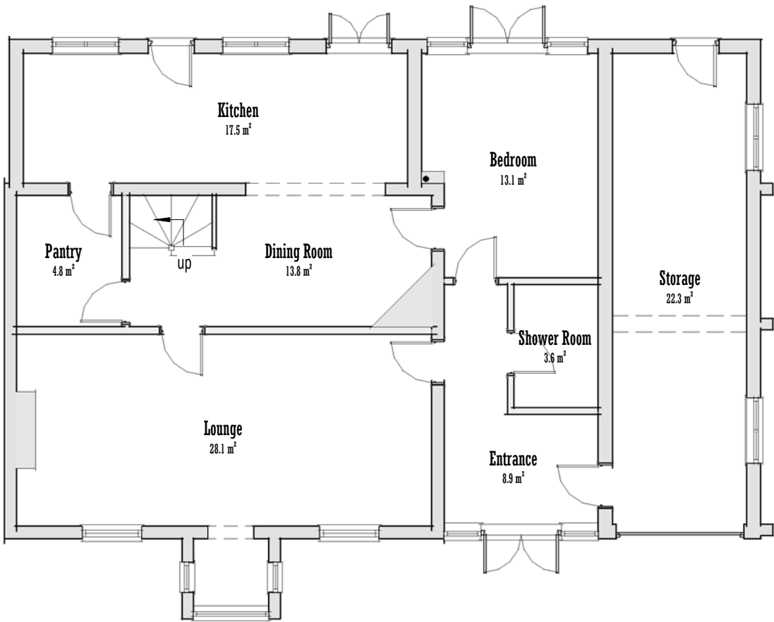
Plan 01 - Ground
