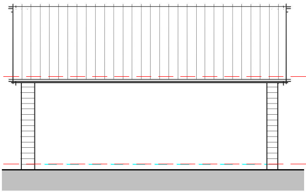
Elevation 01 - Front 1 : 100
