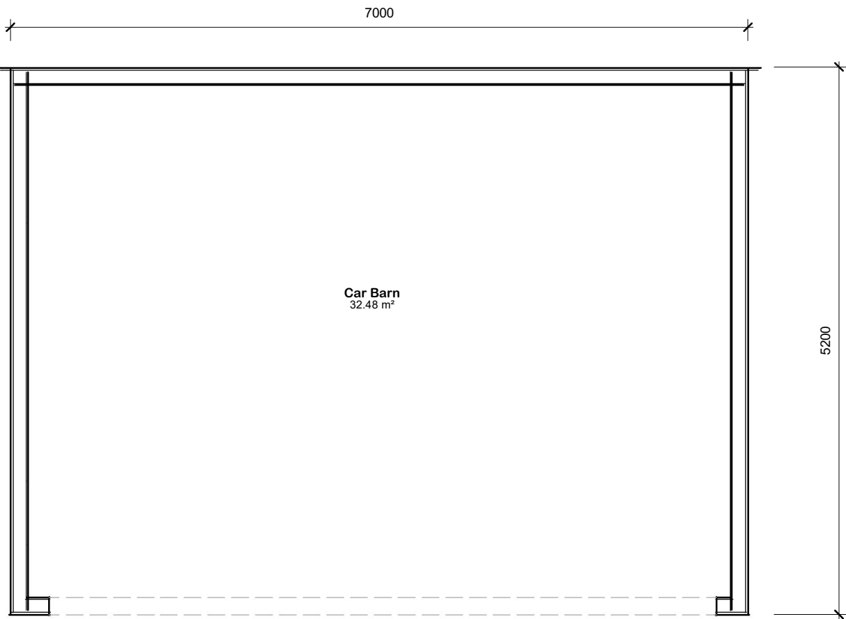
Plan 01 - Ground 1 : 50
