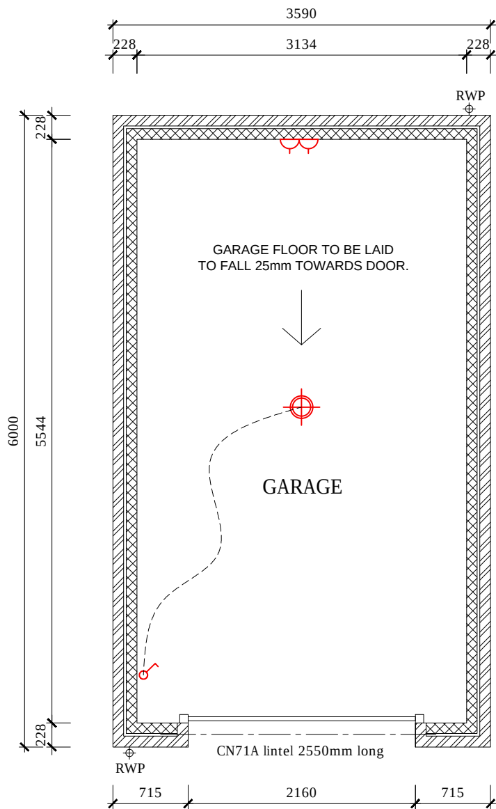
GARAGE PLAN
