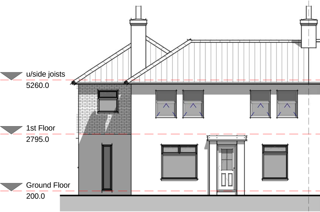
01 - Front Elevation 1 : 100
