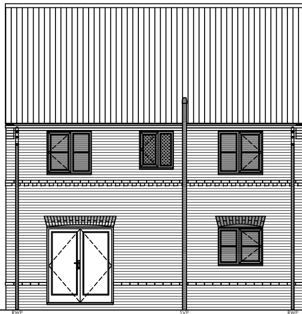
REAR ELEVATION
