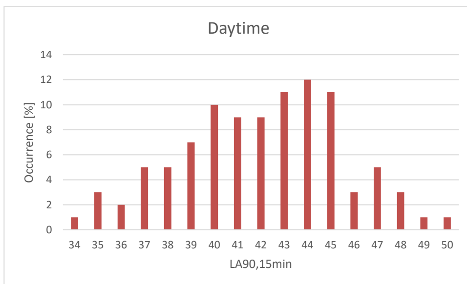
Figure 3: Variation in Daytime Background Noise – South Position 1
