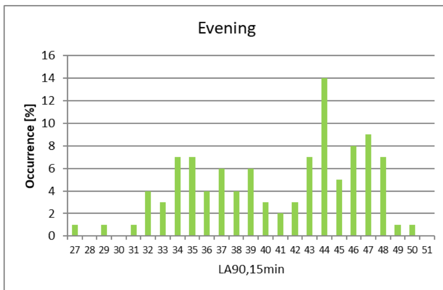
Figure 4: Variation in Evening Background Noise – South Position 1
