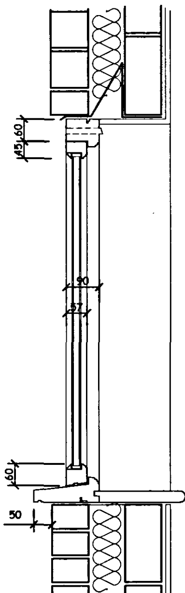
Casement Window Vertical Section 1:10 scale
