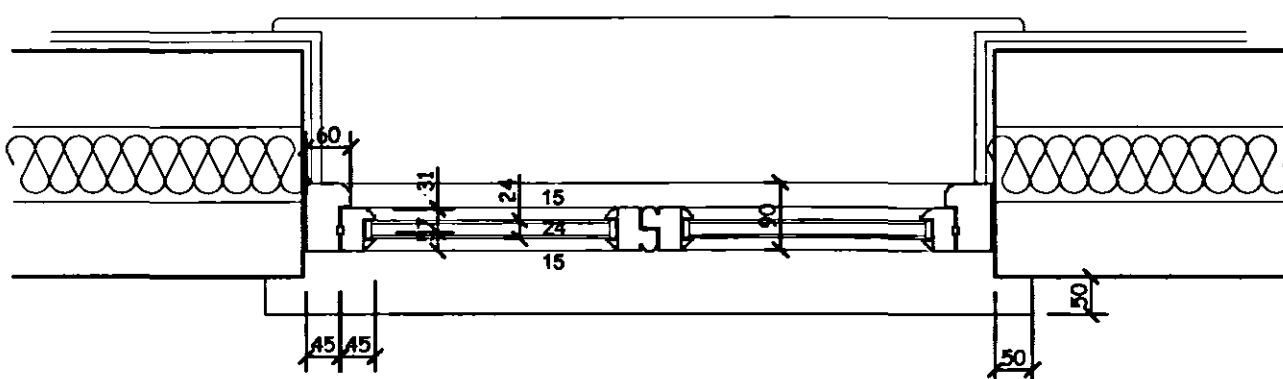
Casement Window Horizontal Plan Section 1:10 scale
