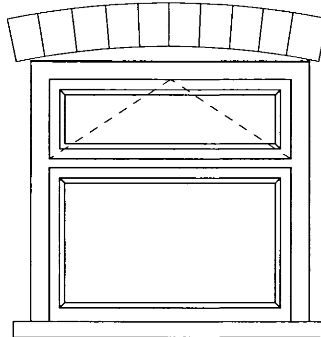
External Elevation
