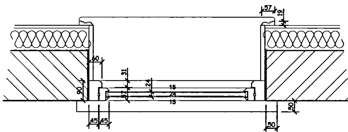
Top Opener Window Horizontal Plan Section 1:10 scale
