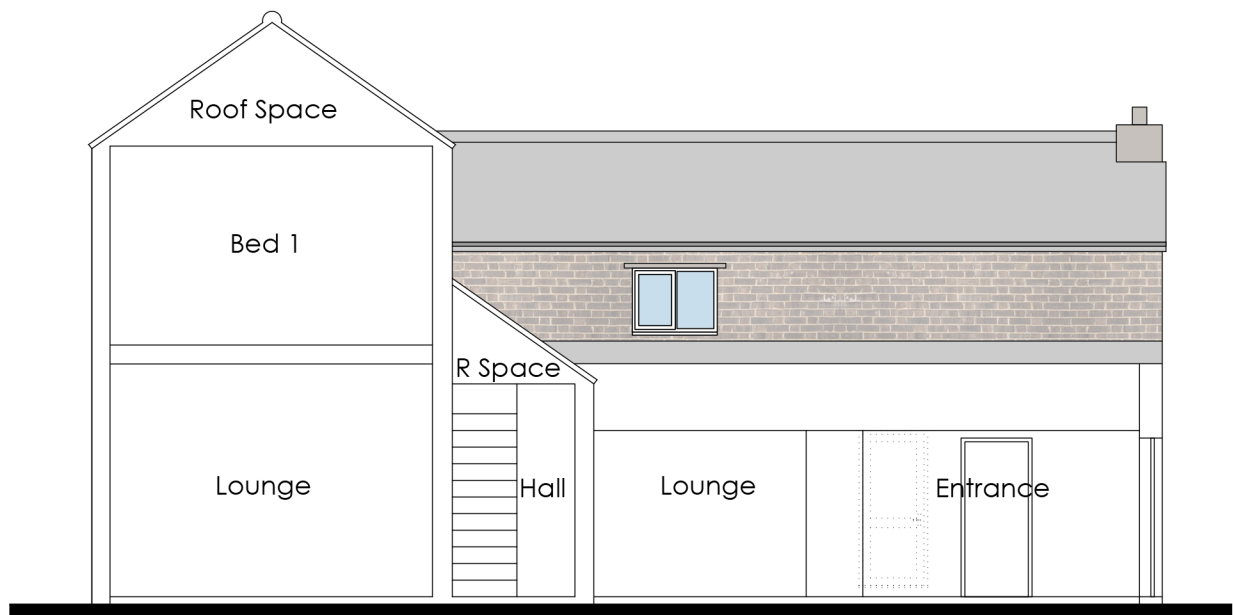
West (Side) Elevation 1:100
