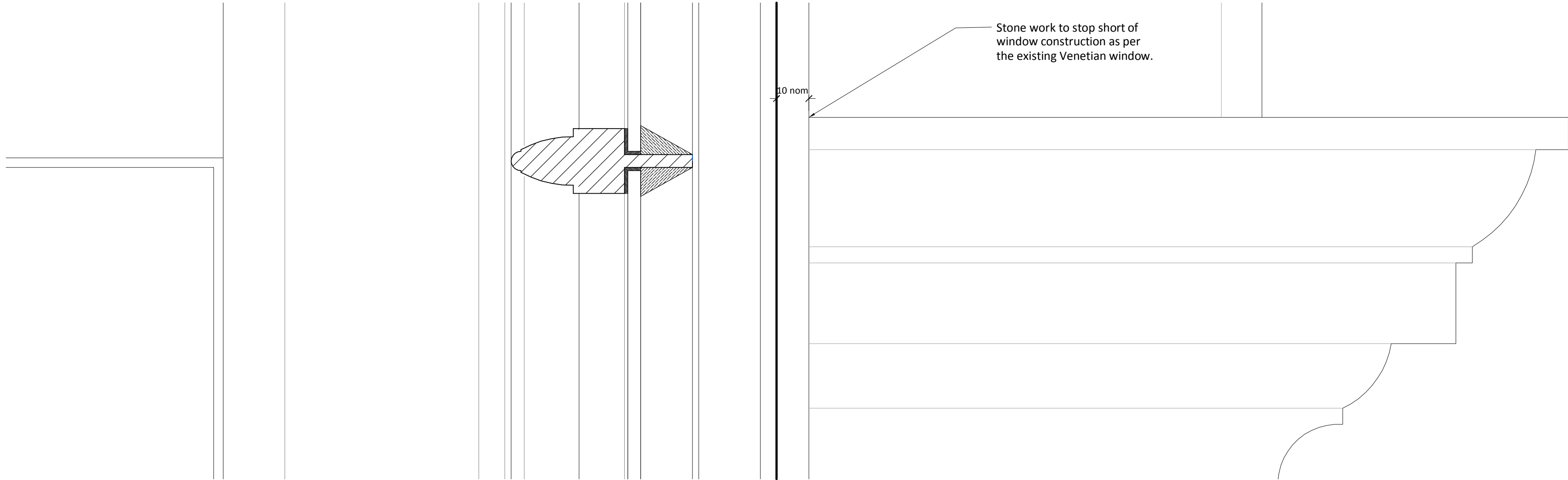
Detail: B Window Bead Scale 1:1
