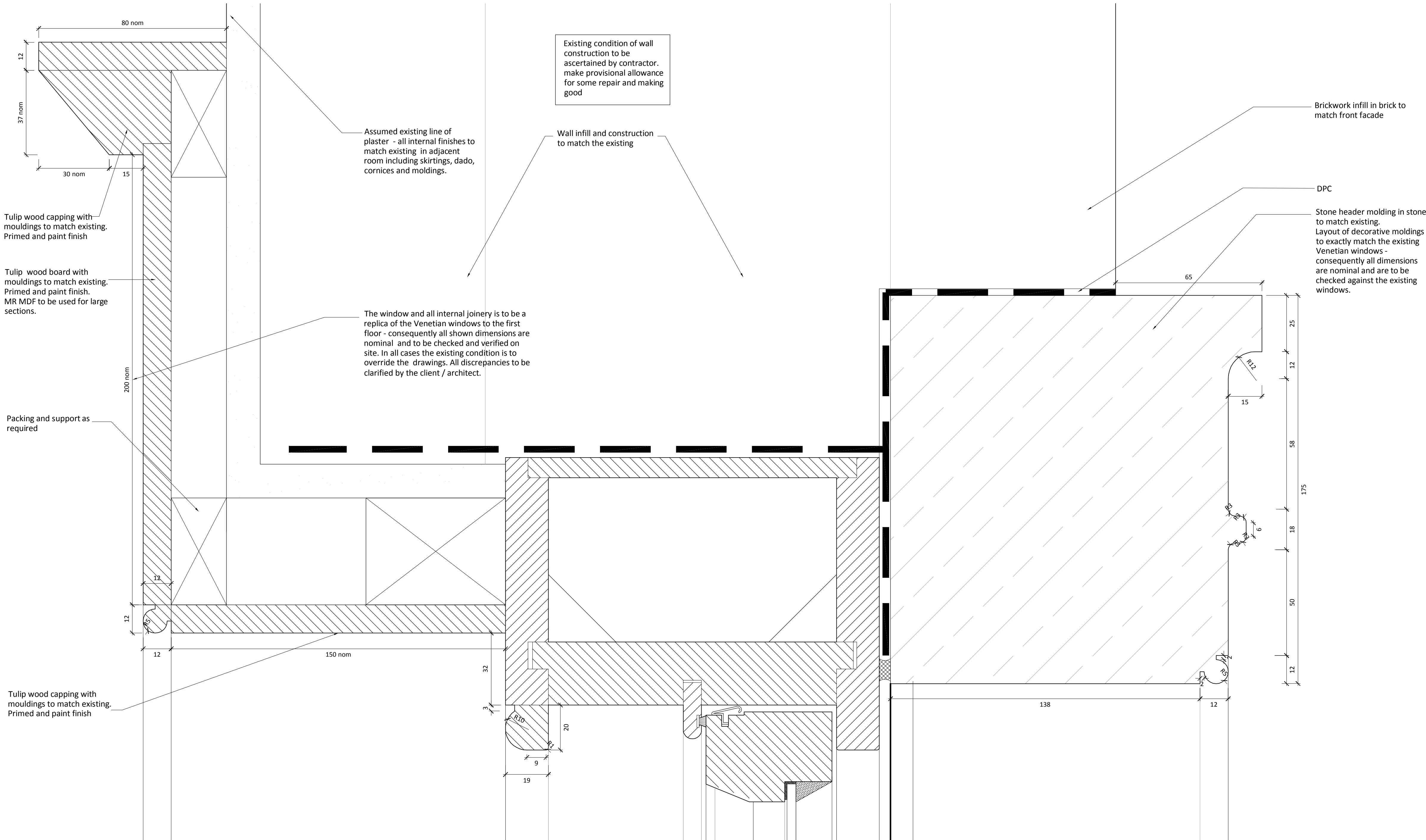
Detail: A Venetian Window Head (Tall) Scale 1:1
