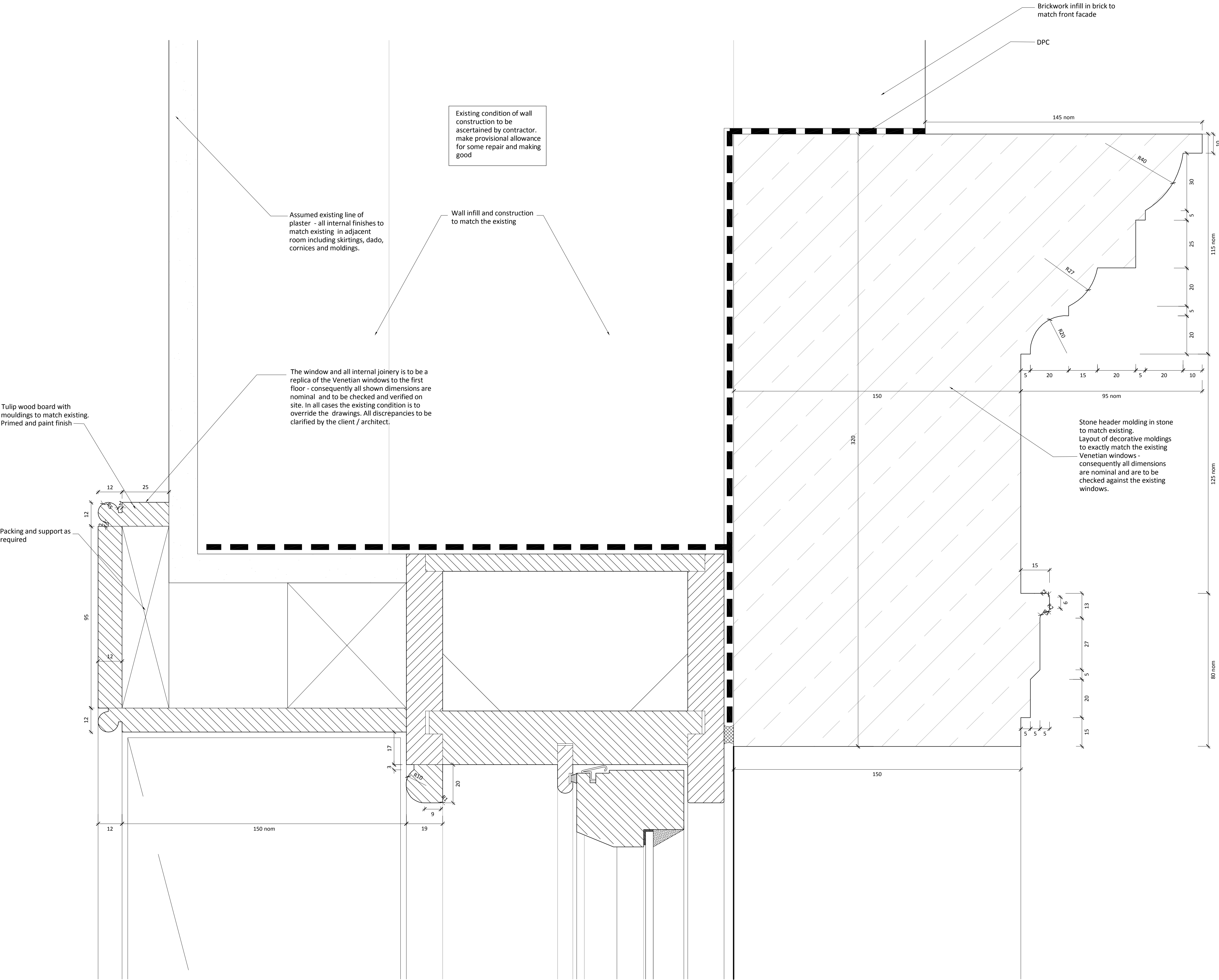
Detail: E Venetian Window Head (Short) Scale: 1:1
