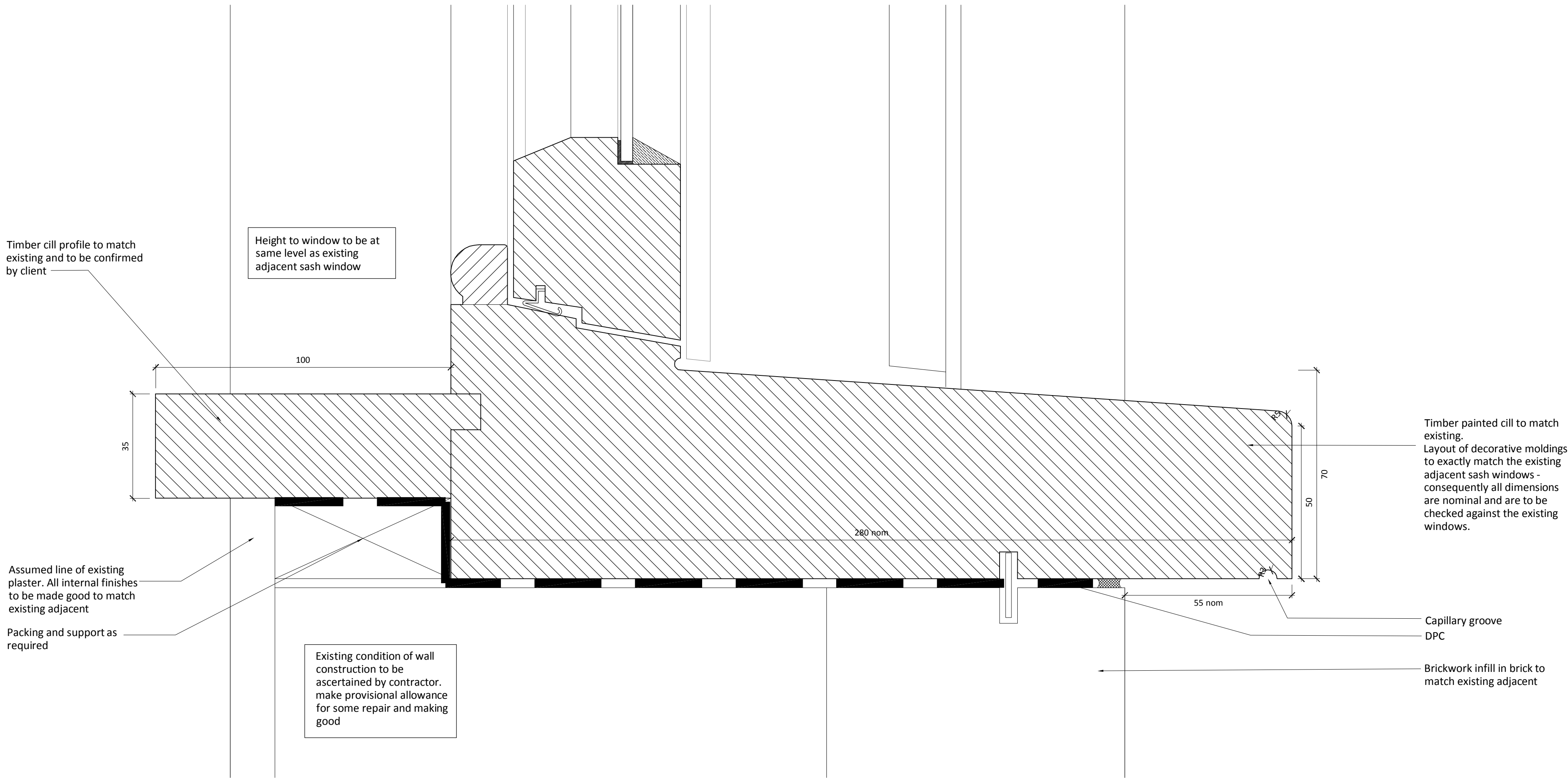
Detail: I Sash Window Cill Scale 1:1
