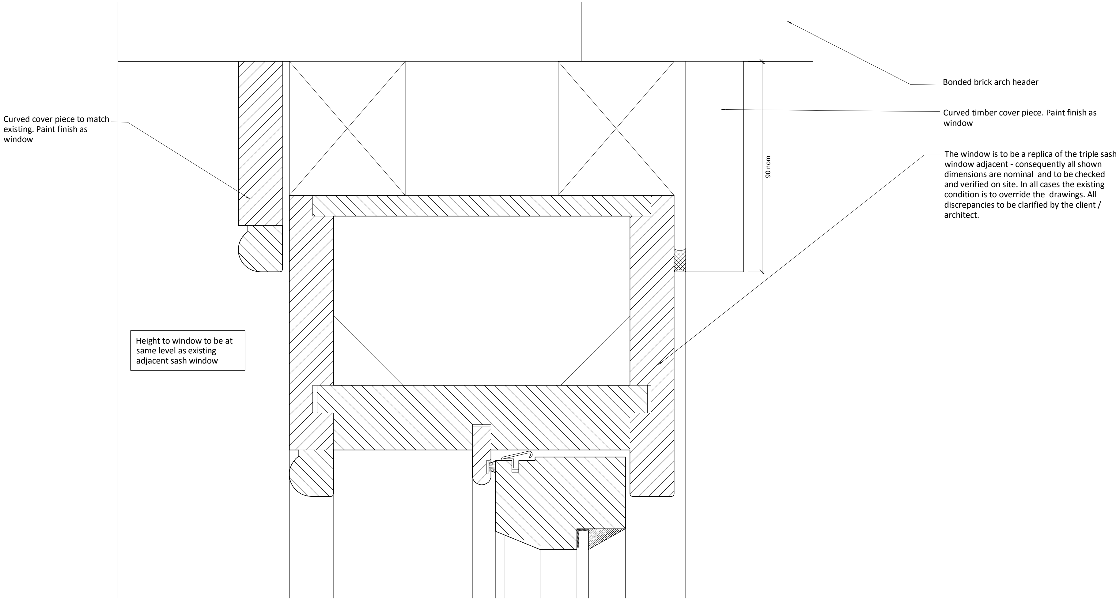
Detail: H Sash Window Head Scale 1:1
