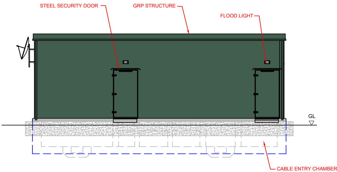
NORTH ELEVATION
