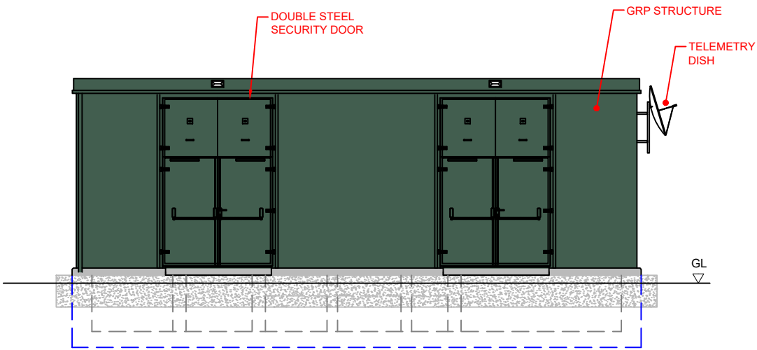
SOUTH ELEVATION
