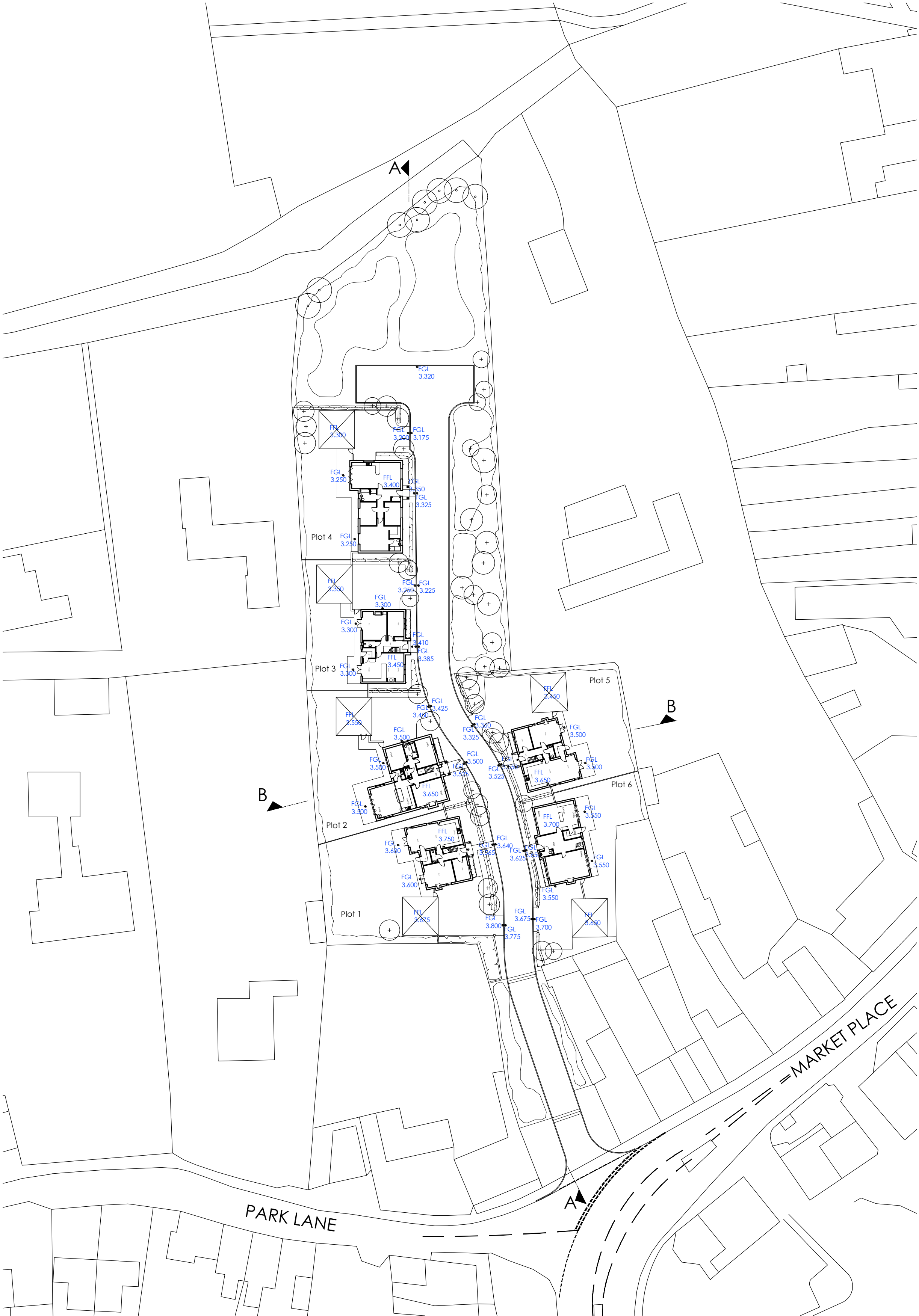
Proposed site levels plan Scale: 1:500 0 5 10 15 20 25 30 35 40 45 50m Scale bar 1:500. N
