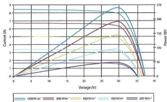
Current-Voltage & Power-Voltage Curve (240S-20)
