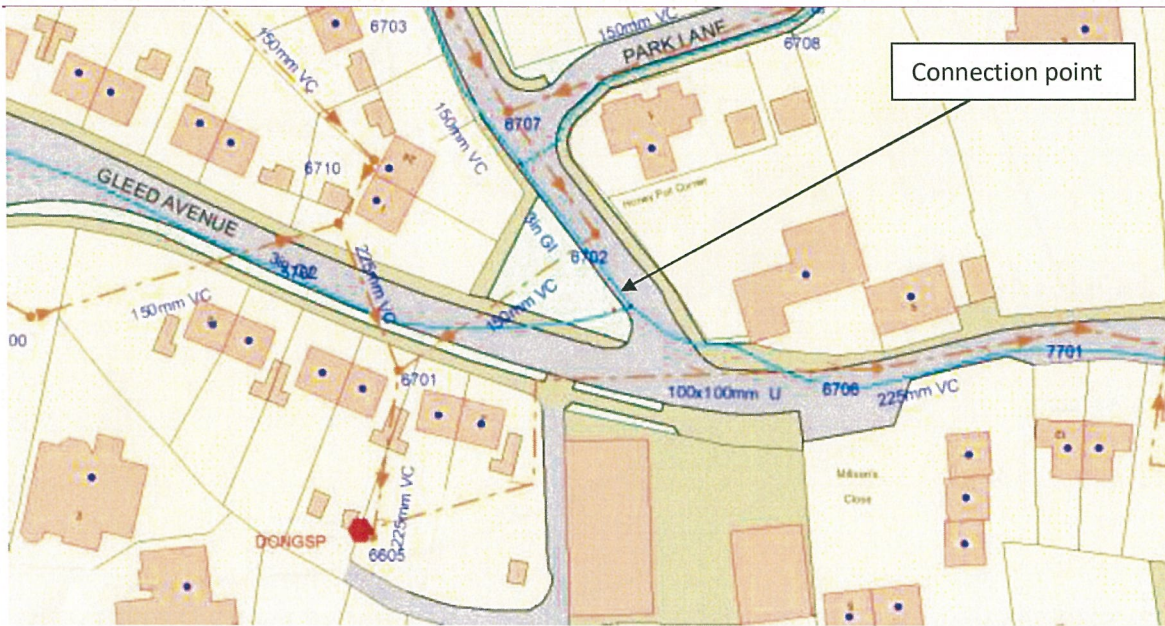
Figure 1: Showing your water point of connection at Park Lane, Donington
