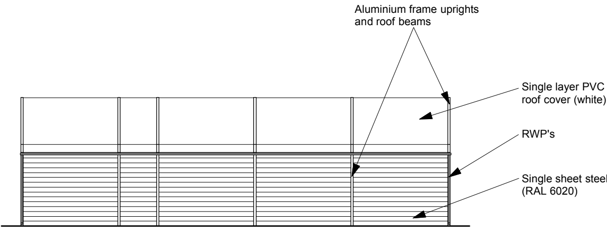
Side Elevation 'A' - 1:200
