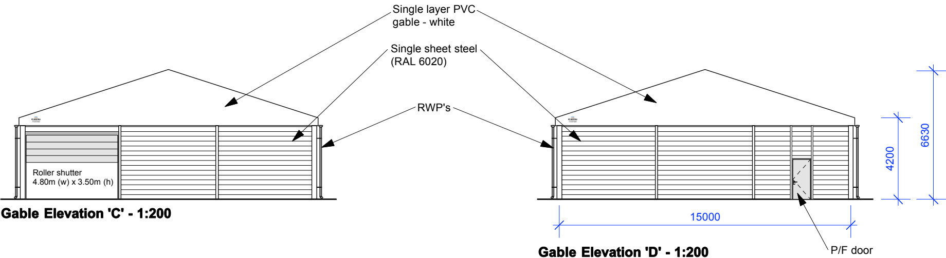
Gable Elevation 'D' - 1:200
