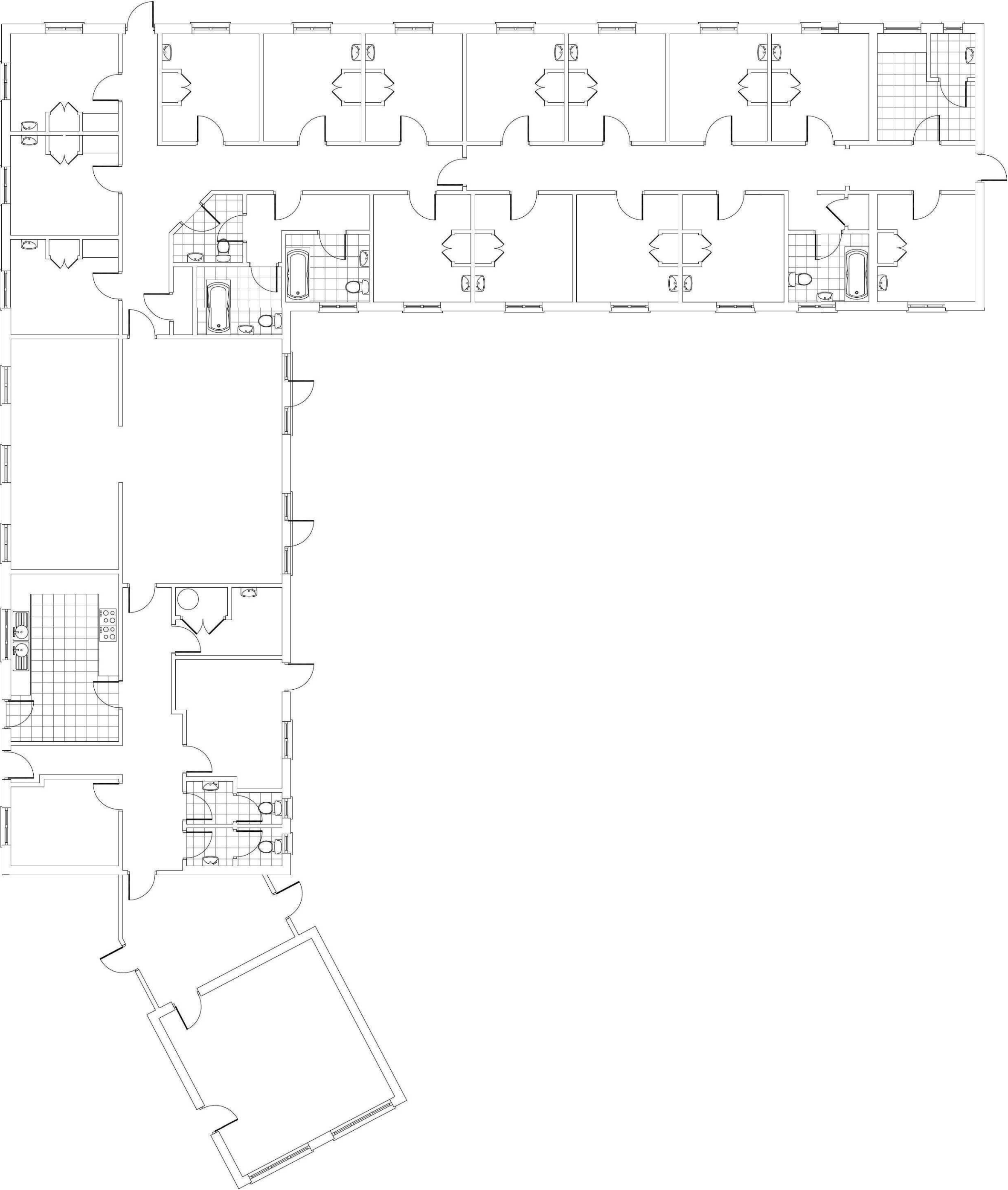
EXISTING GROUND FLOOR LAYOUT 1:100
