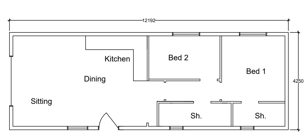
Floor Plan 1:100
