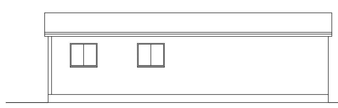
Front Elevation 1:100 Side Elevation 1:100
