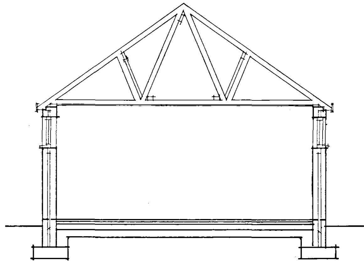
SECTION
