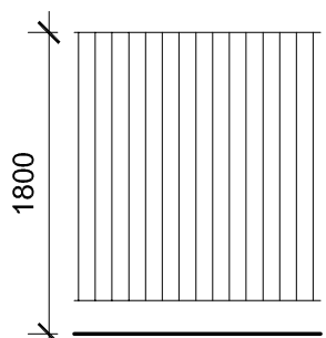
Close Boarded Fence
