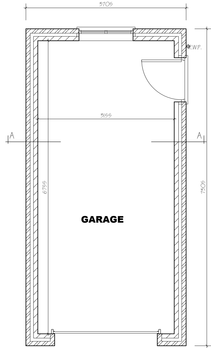
FLOOR PLAN - GARAGE - PLOT'S 1, 2, 4 & 5
