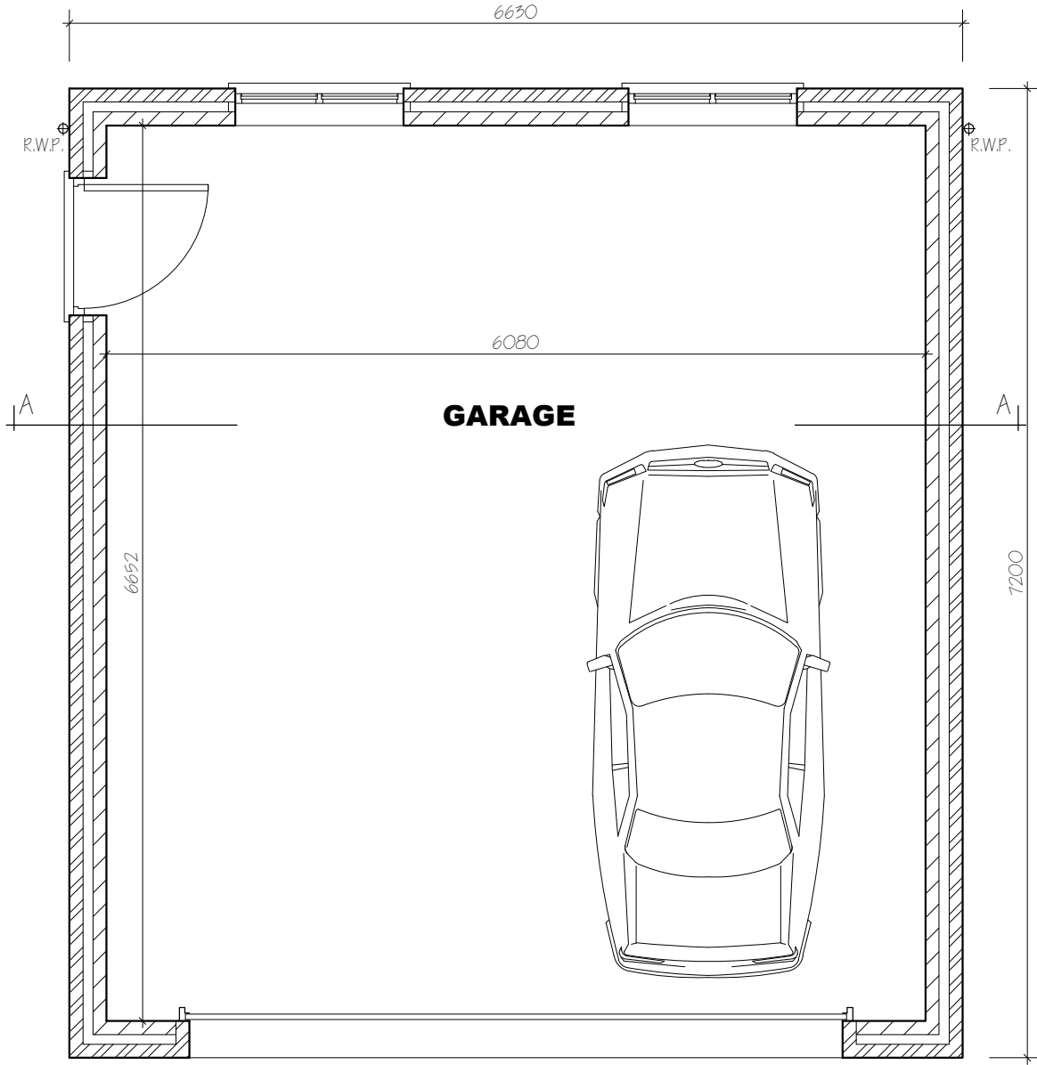
FLOOR PLAN - GARAGE - PLOT 3
