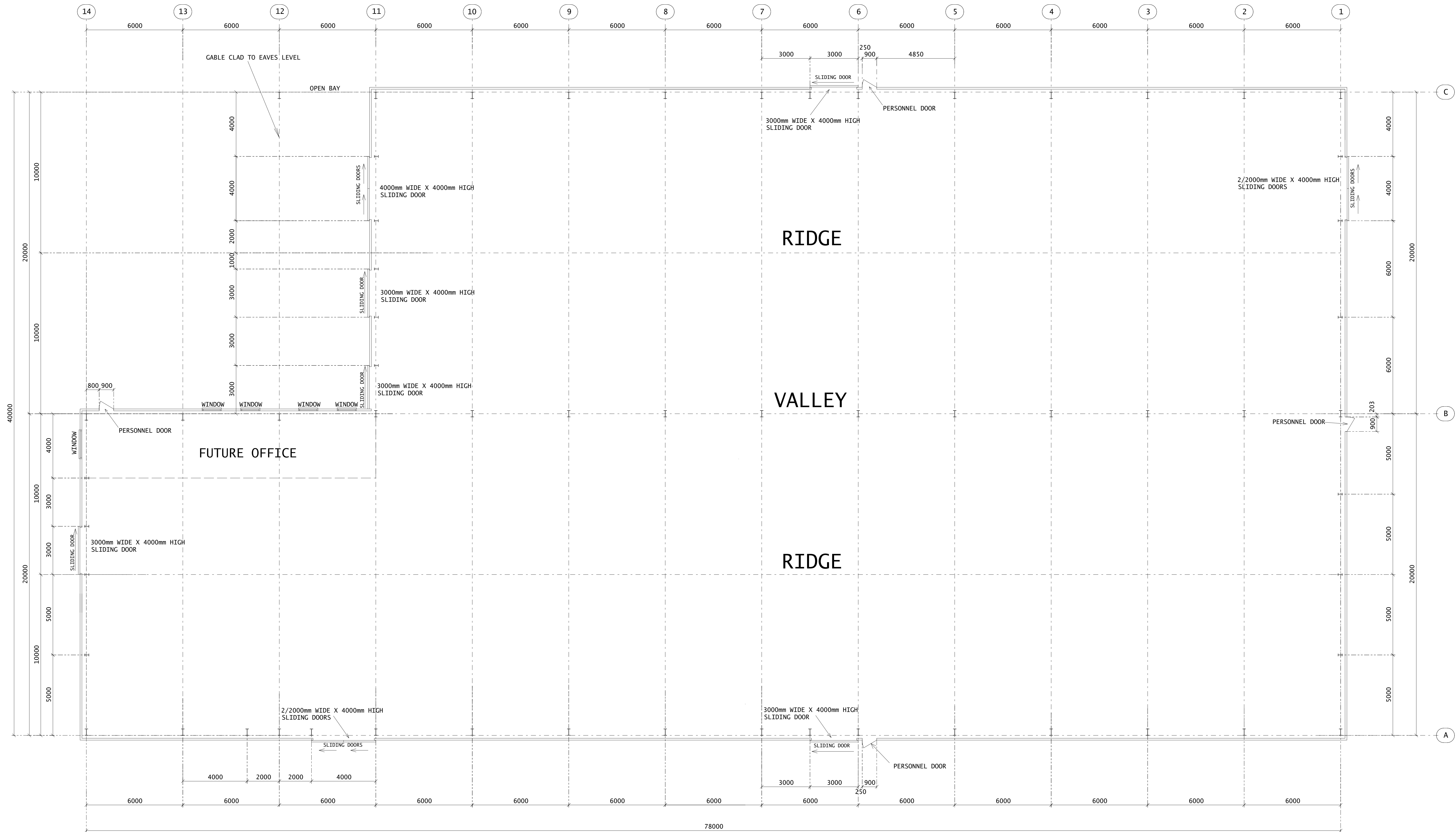
PLAN (SCALE 1:100)
