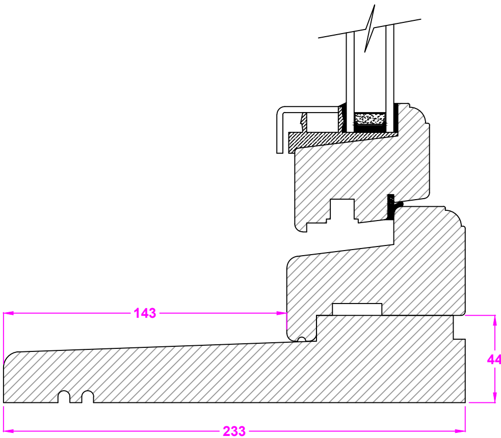
SECTION THROUGH BOTTOM OF A PRESTIGE HARDWOOD/ NORDIC PINE CASEMENT WINDOW WITH A 233mm CILL
