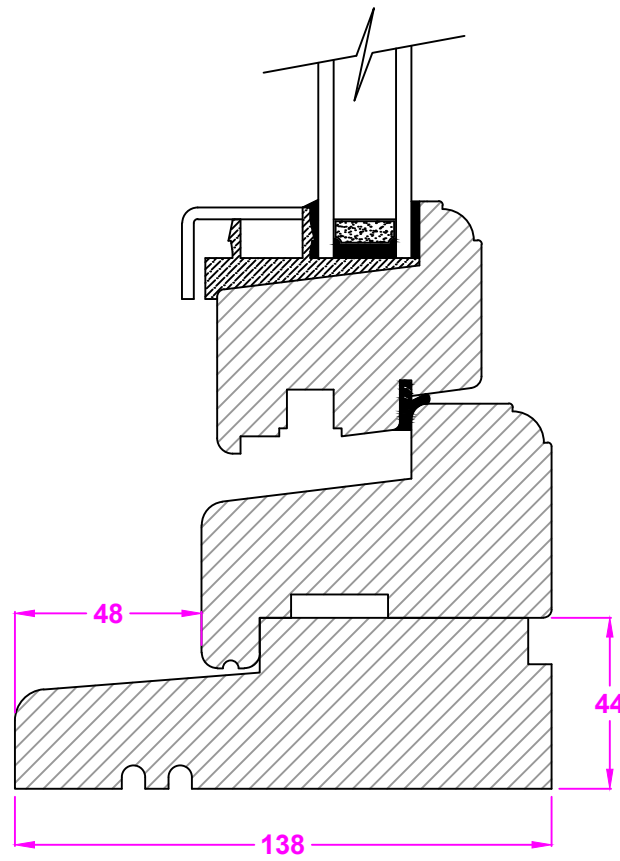
SECTION THROUGH BOTTOM OF A PRESTIGE HARDWOOD/ NORDIC PINE CASEMENT WINDOW WITH A 138mm CILL
