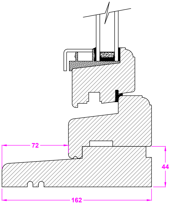
SECTION THROUGH BOTTOM OF A PRESTIGE HARDWOOD/ NORDIC PINE CASEMENT WINDOW WITH A 162mm CILL
