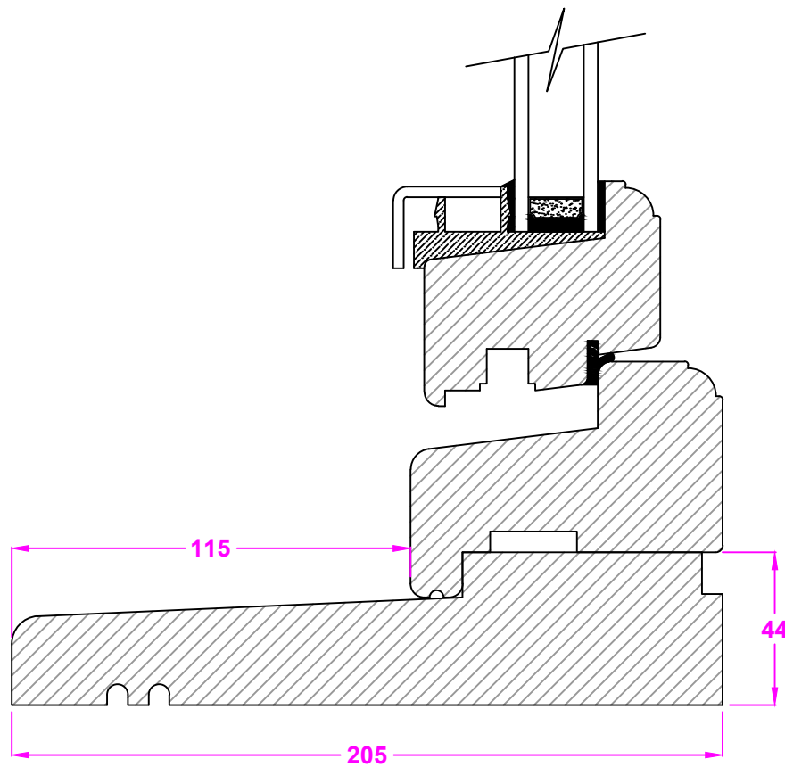
SECTION THROUGH BOTTOM OF A PRESTIGE HARDWOOD/ NORDIC PINE CASEMENT WINDOW WITH A 205mm CILL
