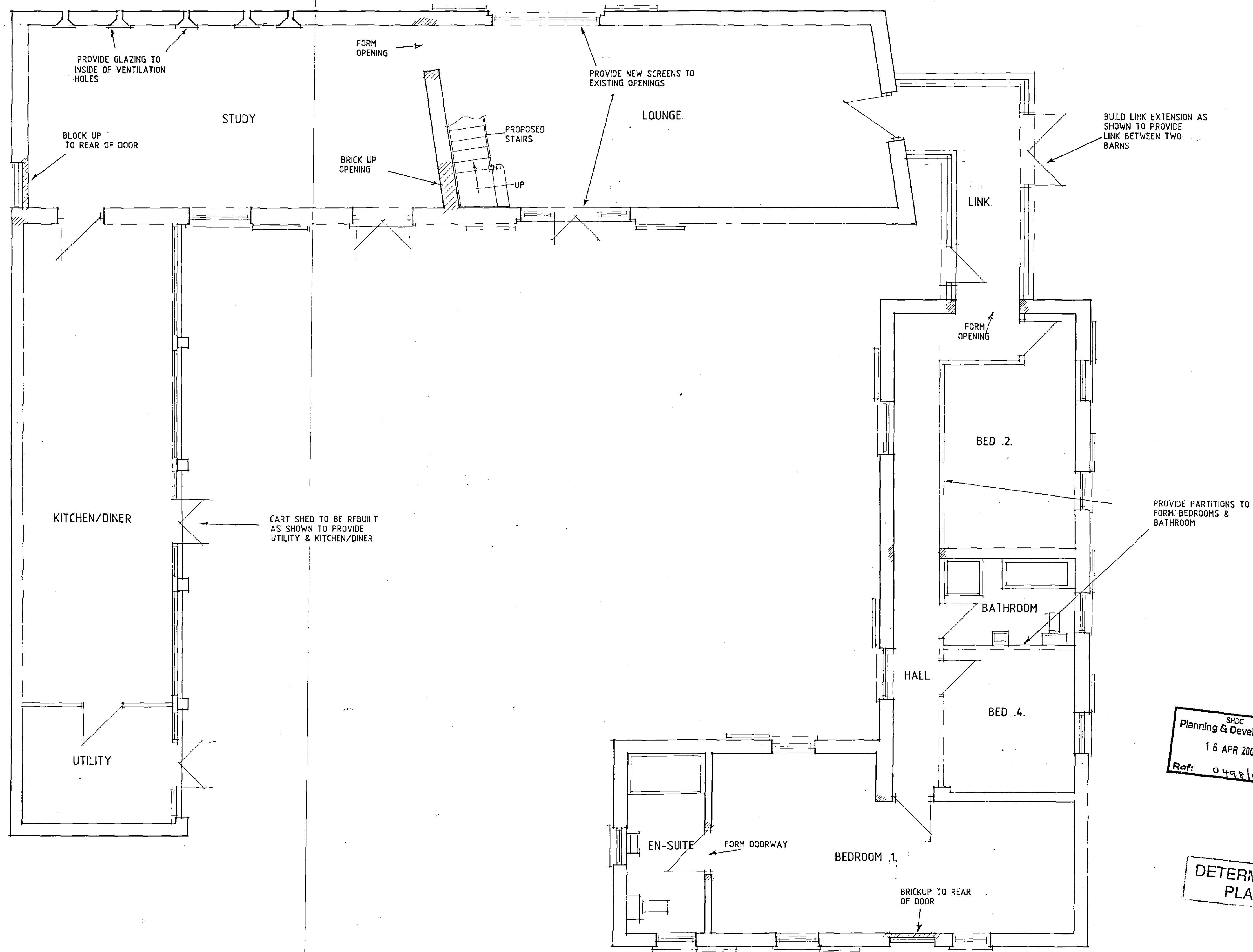
PROPOSED GROUND FLOOR PLAN
