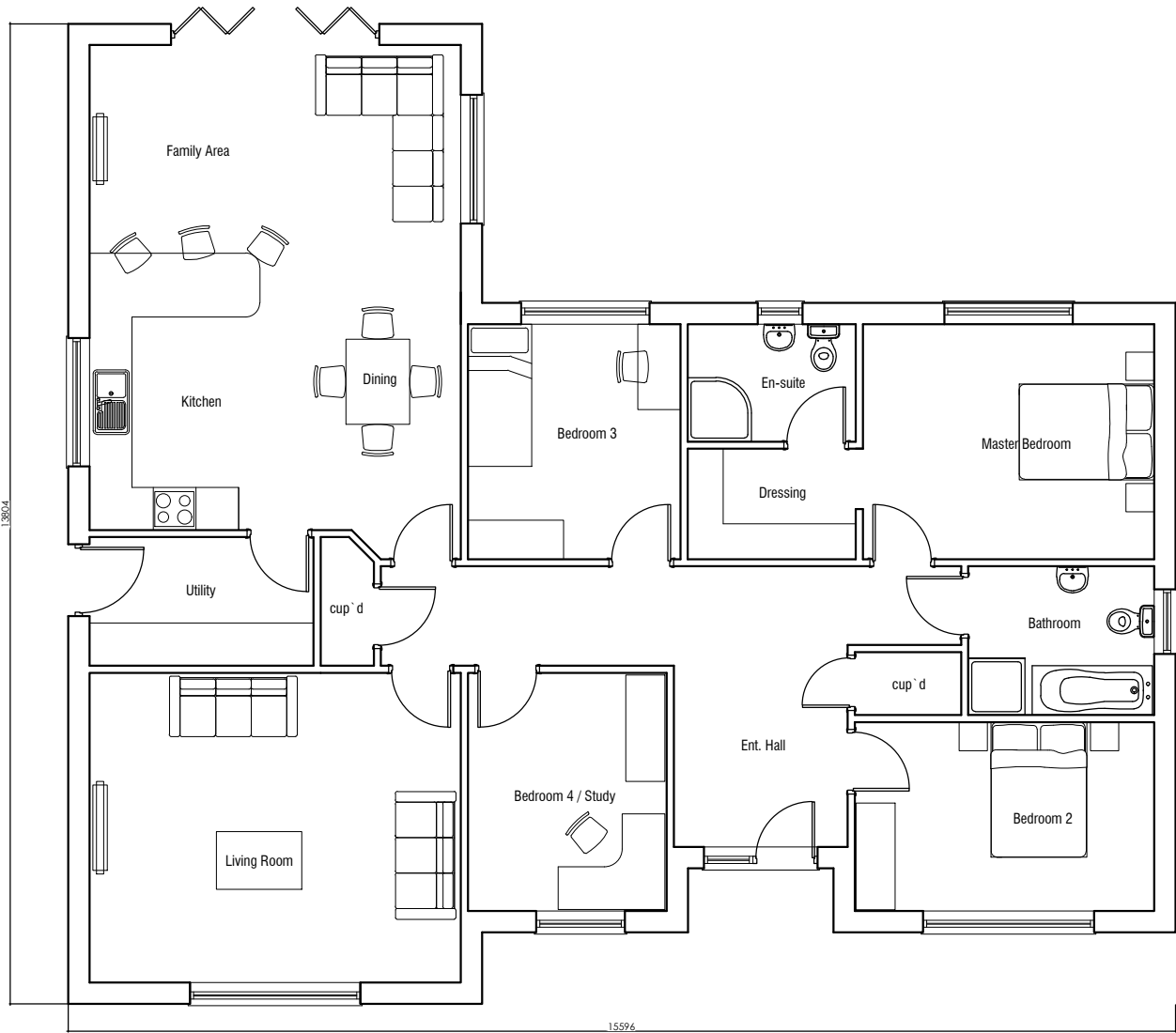
Plot 2 Floor Layout 147.35m² / 1586.1ft² (Internal Blockwork)
