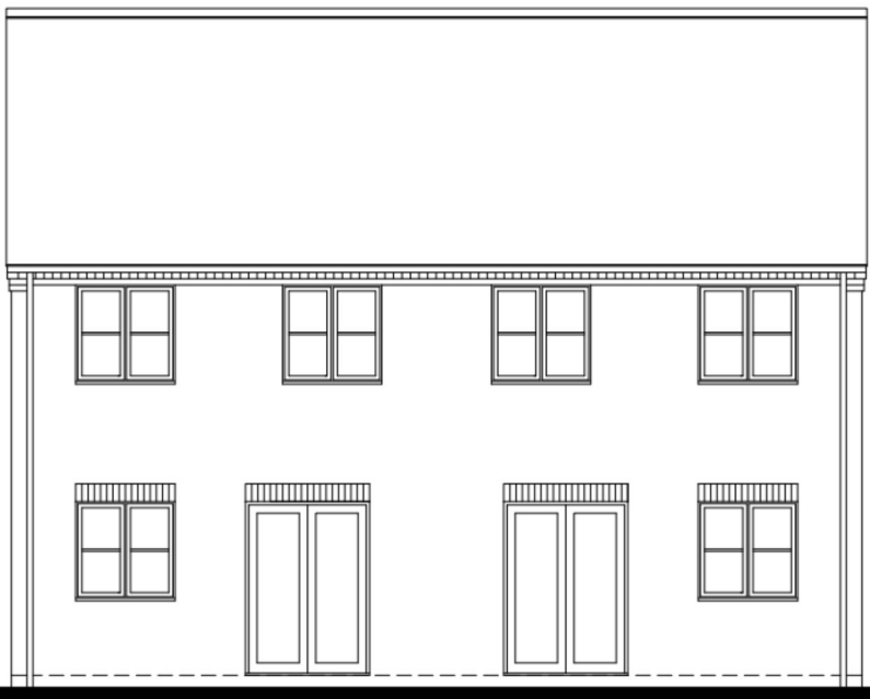
Rear Elevation
